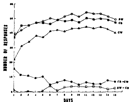
Figure 1. Stroop Test: Group means for black and white words (BW), color blocks (CB), color words (CW), BW-CB, and CB-CW over 15 days (n=19).
