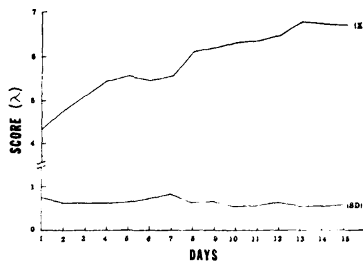
Figure 12. Critical Tracking Test: Group means ( \bar{X} ) and standard deviations (SD) over 15 days ( n=18 ).
