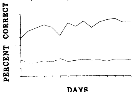
Figure 7. Interference Susceptibility means and standard deviations for percent correct across 15 days (n=23).
