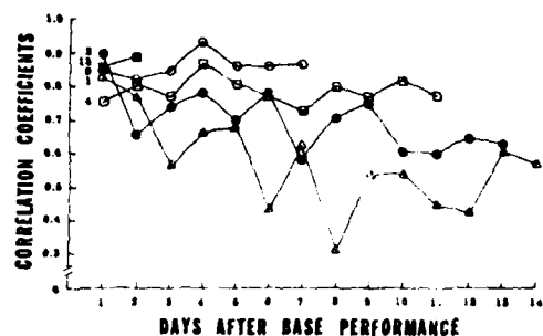
Figure 5. Stroop Test: CW reliabilities for selected base days (1, 2, 4, 9 & 13) and those following over 15 days (n=19).
