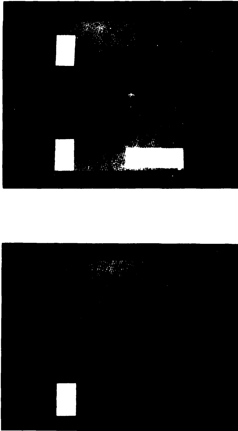
FIGURE 57 X-RADIOGRAPHS OF SPECIMEN 8-8 (PENETRANT ENHANCED) SHOWING THE INITIAL AND FINAL CONDITION AFTER ROOM TEMPERATURE EXPOSURE TO TETRABROMOETHANE
