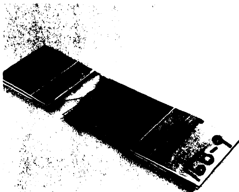
FIGURE 121 SPECIMEN 16B-9 AFTER FATIGUE FAILURE
