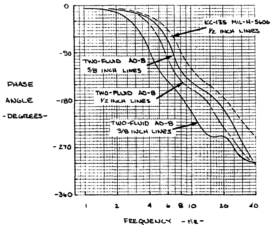
Figure 3.12 Effect of Line Diameter on Frequency Response
