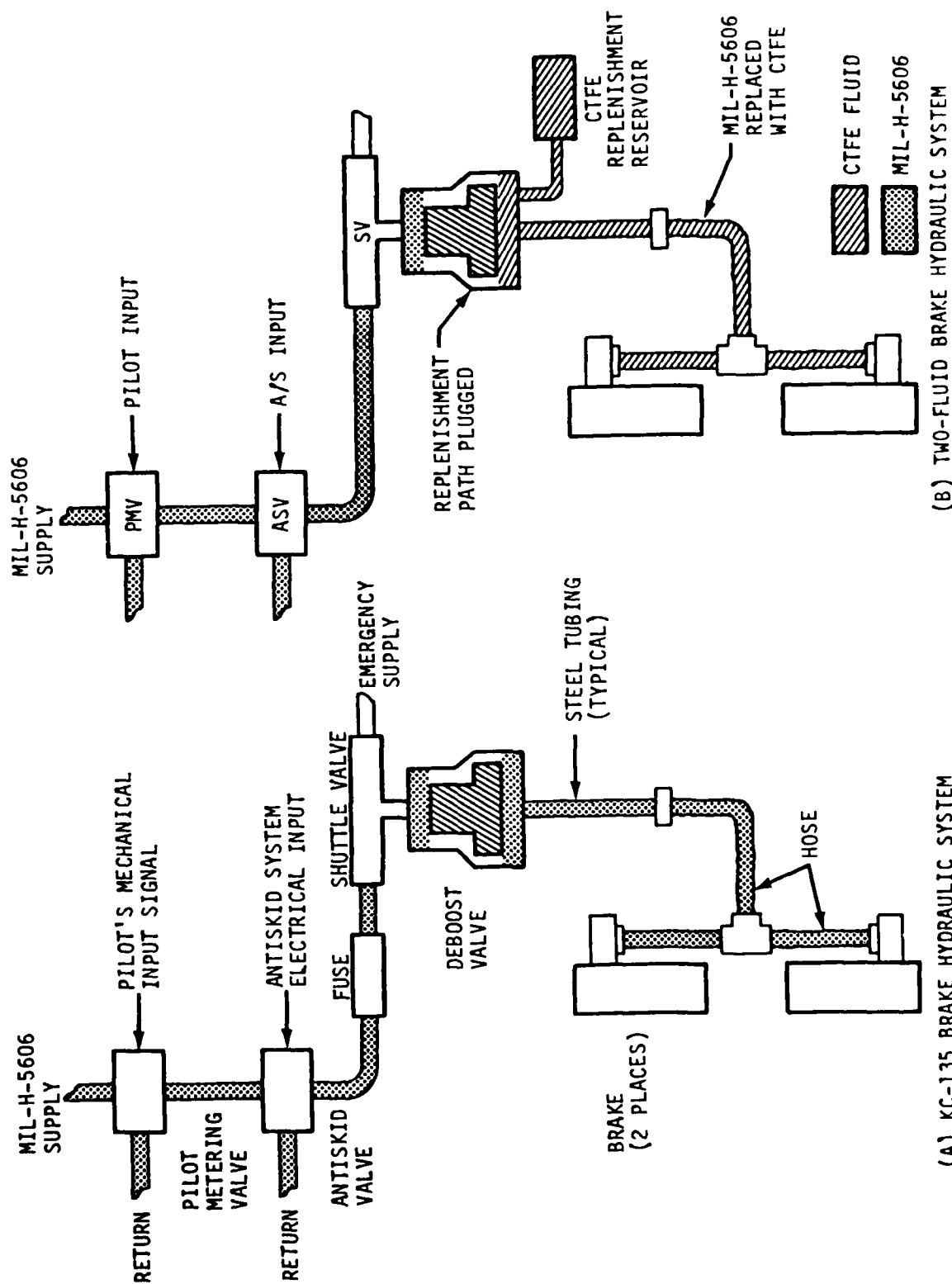
Figure 10 Two-Fluid Brake Hydraulic System
