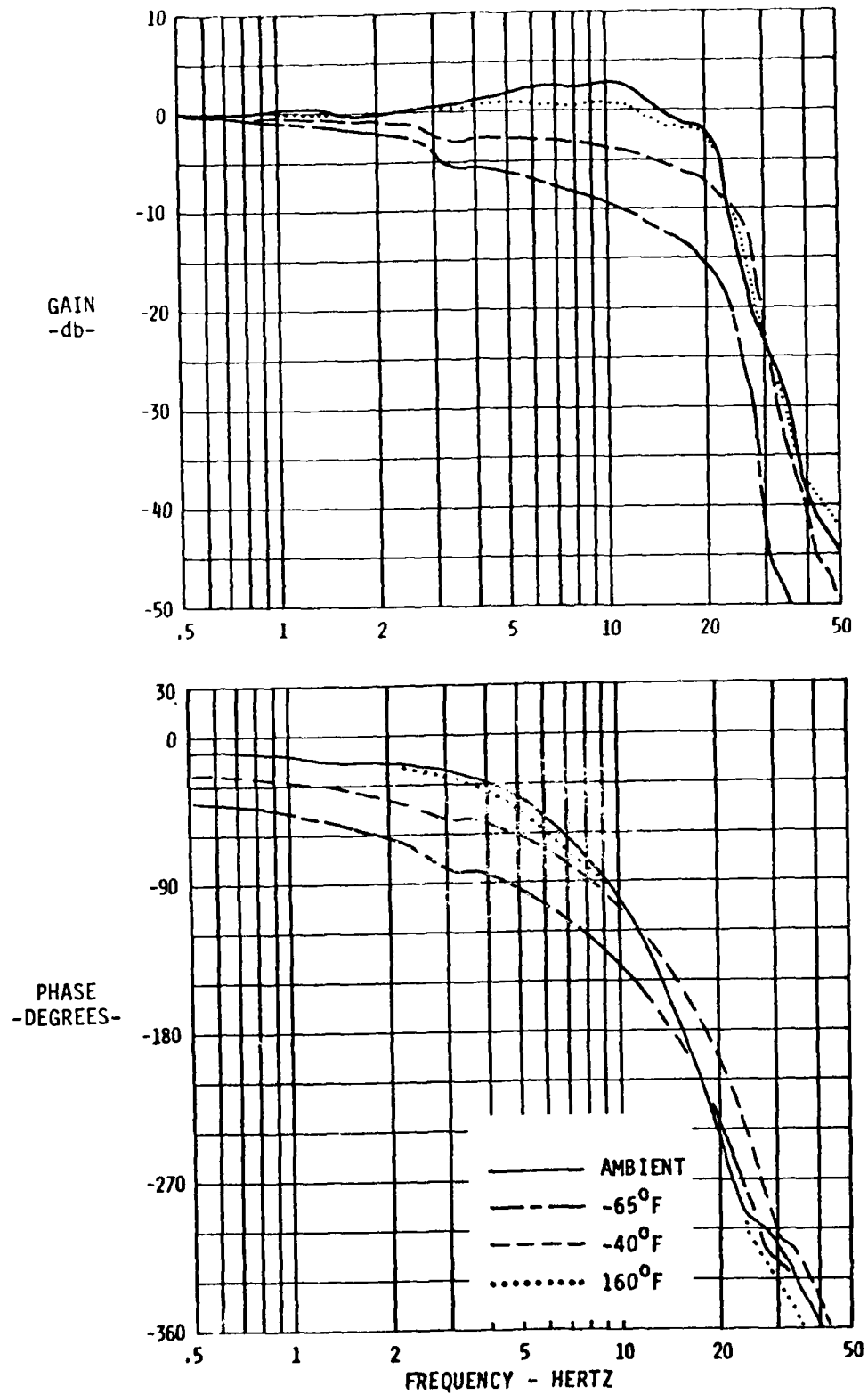
Figure E-12 Frequency Response, Standard Brake System, 66% \pm 100 psi 245
