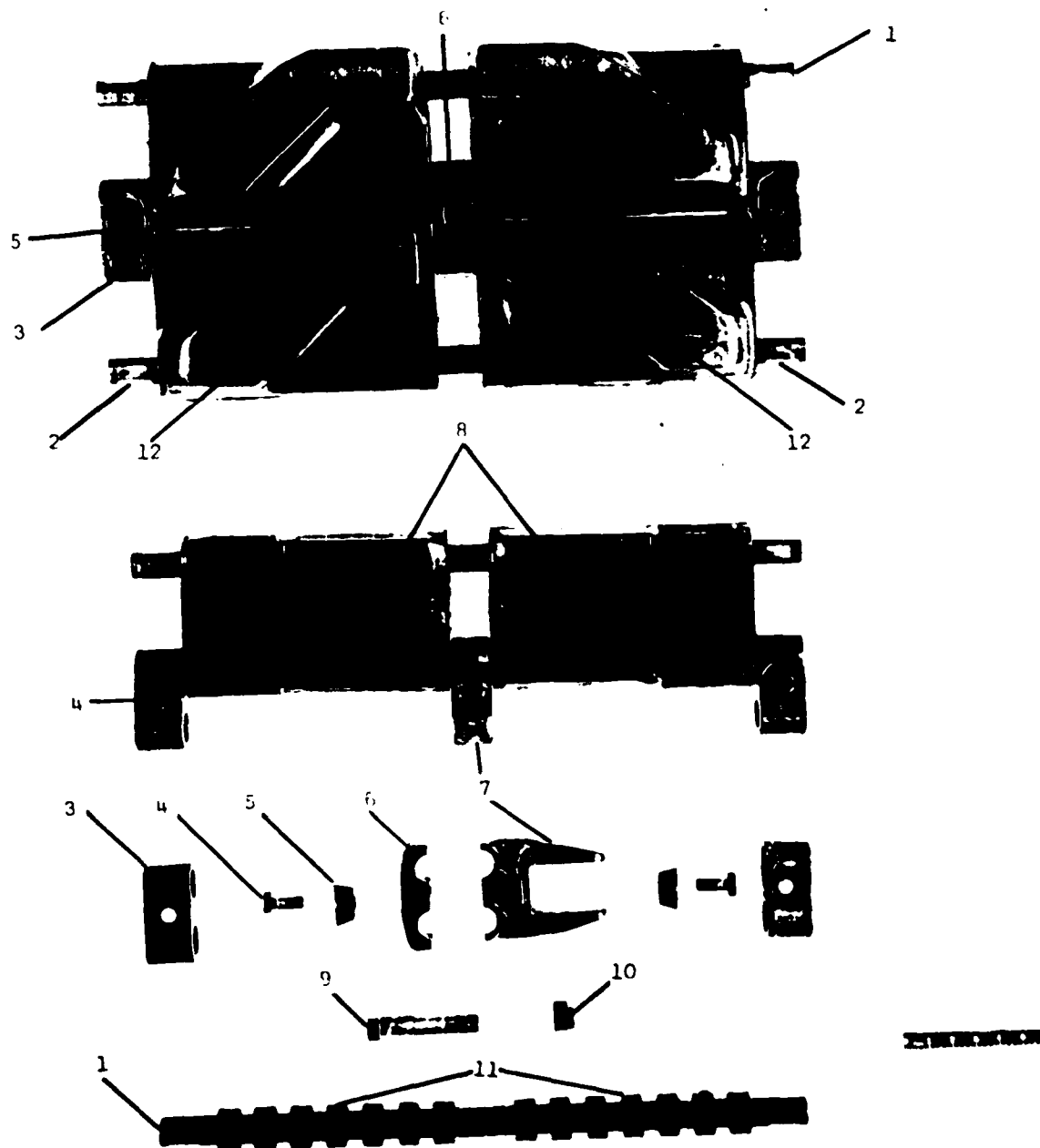
T97E2 TRACK
