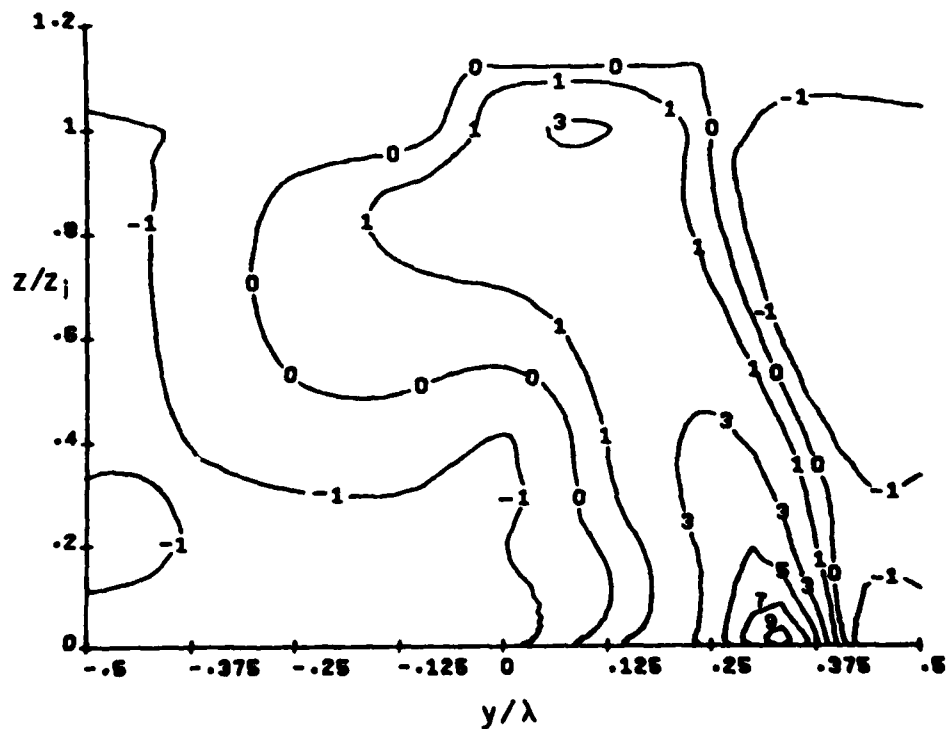
Figure 5.2.4 - Roll species contours for the conditions of Figure 5.2.2. The normalizing maximum value is \Delta C_{\max} w_0 / \overline{Cw_0} = 6.62 .
