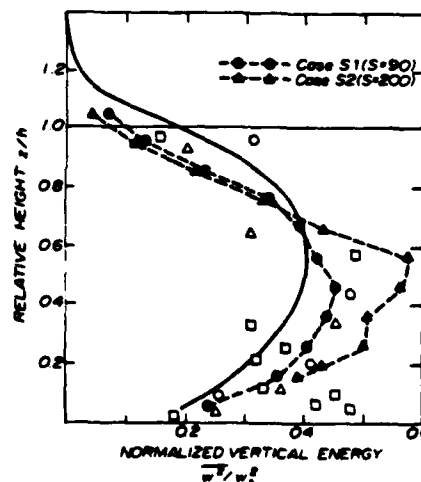
Figure 3.3.6 - Vertical velocity fluctuations as calculated by Zeman and Lumley (1976) compared with data: solid circles and triangles, Willis and Deardorff (1974); open circles and triangles, Lenschow (1970, 1974) and Lenschow and Johnson (1968); and squares, Telford and Warner (1964).
