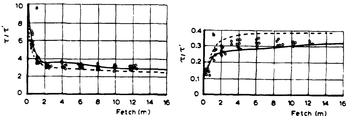
Figure 5.1.1 - Response of surface shear to step change in surface roughness. Lewellen (1977) (—); Rao, et al. (1974) (---). Data from Bradley (1968). (a) Smooth to rough z_0 = 0.002 cm, z_0 = 0.25 cm; (b) rough to smooth z_0 = 0.25 cm, z_0 = 0.002 cm.
