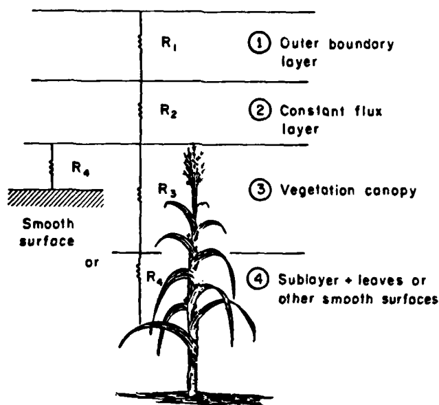
Figure 6.4.2 - Four different regions of the planetary boundary layer for study of the aerodynamic resistance to \text{SO}_2 deposition.
