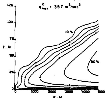
Figure 4.6.5 - Turbulence ( q^2 ) distribution in advective-radiative fog of Figures 4.6.3 and 4.6.4.
