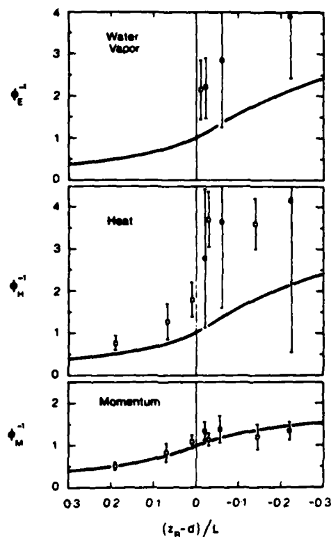
Figure 3.6.3 - Stability dependence of inverse influence functions \phi_{H,E}^{-1} , measured over Thetford forest ( \square ) and Uriarra forest ( \blacksquare ). The smooth curves represent typical inertial-sublayer behavior. Raupach and Thom (1981).
