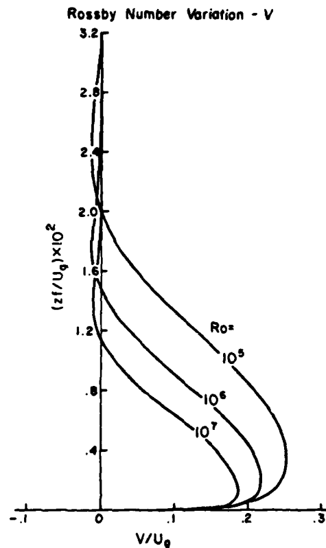
Figure 3.2.2 - Influence of Rossby number on the mean wind component in the direction normal to the geostrophic wind for the conditions of Figure 3.2.1.
