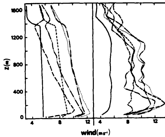
Figure 4.1.6 - Comparison of model calculations by Andre, et al. (1978) with Wangara data. Computed (left) and observed (right) profiles of mean horizontal wind during Night 33-34: —, t = 18 h; ----, t = 21 h; ····, t = 00 h; ·-·-·, t = 03 h; - - - - -, t = 06 h; - · - · - , t = 08 h.
