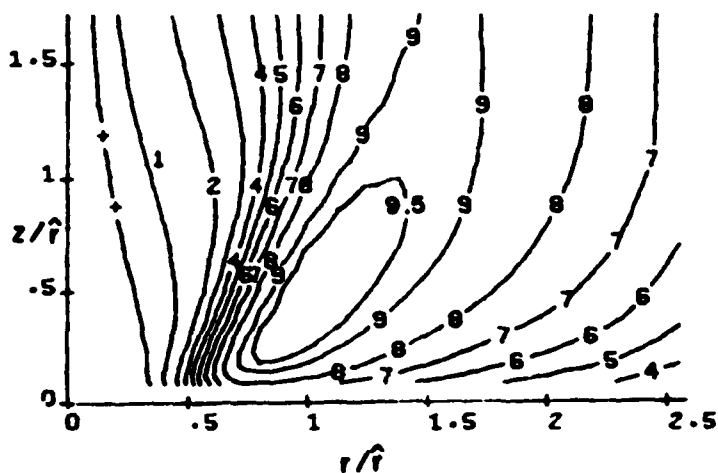
Figure 5.4.1 - Mean tangential velocity contours as predicted by an axisymmetric tornado model. Contours labeled in tenths of maximum V , and radial and vertical coordinates normalized by the radius at which V_{\max} occurs.
