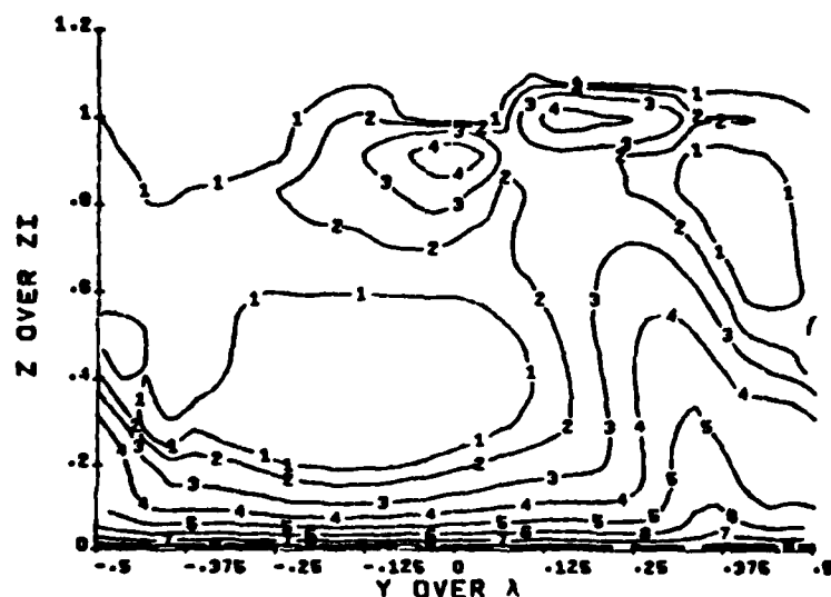
Figure 6.3.2 - Contours of the radar refractivity structure function ( C_n^2 ) within the roll vortices predicted by a model run with T(\text{sea surface}) = 20^\circ\text{C} , U_0 = 10 \text{ m/sec} , z_i/L \approx -10 , \alpha = -10^\circ , \partial\theta/\partial z(\text{above inversion}) = 0.01 \text{ C/m} , \Delta h(\text{inversion}) = 2.5 \text{ g/Kg} . Contours labeled n denote 2^{(n-7)} \times 10^{-12} so that there is a factor of 2 difference between each of the contours.
