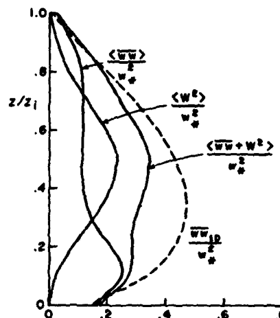
Figure 5.2.6 - Comparison between the one-dimensional and two-dimensional predictions for vertical velocity variance. For the two-dimensional calculation, the y-averaged, large scale roll contribution is denoted by \langle \overline{w} \rangle and the smaller scale turbulence by \langle w^2 \rangle .
