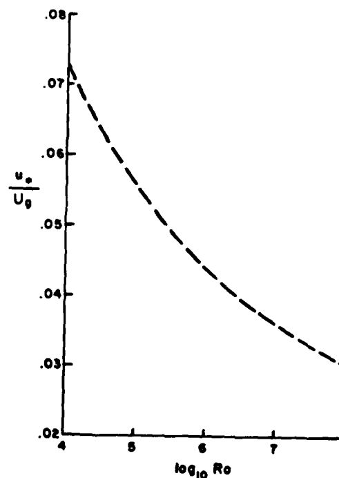
Figure 3.2.4 - Surface shear stress as a function of Rossby number for the neutral planetary boundary layer.
