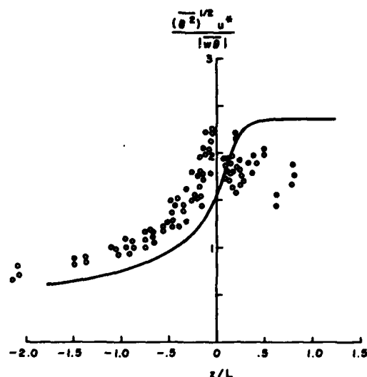
Figure 3.1.3 - Temperature fluctuation in the atmospheric surface layer. Model calculation from Lewellen and Teske (1973). Data from Wyngaard, et al. (1971).
