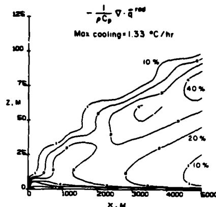
Figure 4.6.4 - Radiative cooling distribution in advective-radiative fog. Note shift of maximum cooling rate away from surface to top of cloud bank as fog bank becomes radiatively thick ( \delta \geq \lambda_{\text{rad}} ). Oliver, et al. (1978).
