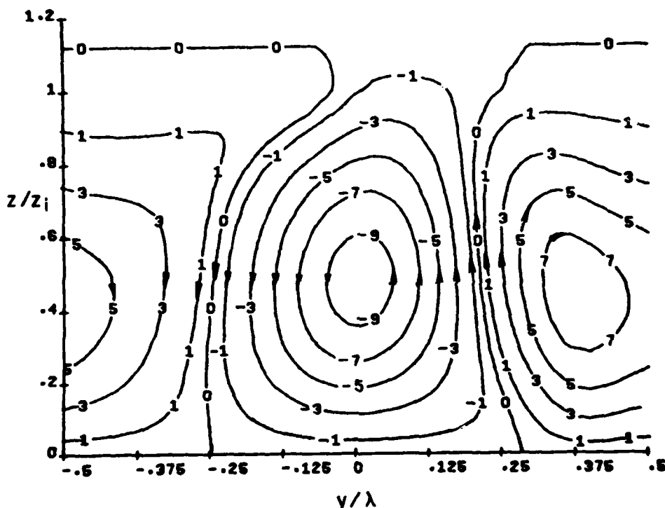
Figure 5.2.2 - Roll stream function contours for the example case of \alpha = -10^\circ , \lambda/z_i = 3 , L/z_i = -0.1 . The profiles are normalized by a maximum value \Delta\psi_{\max}/w_* z_i = 0.287 ( \Delta\psi = \psi - \langle \psi \rangle ), with \pm 9 denoting \pm 90\% of maximum value; \pm 7 , \pm 70\% , etc. The arrows indicate flow direction. (Lewellen, et al., 1980).
