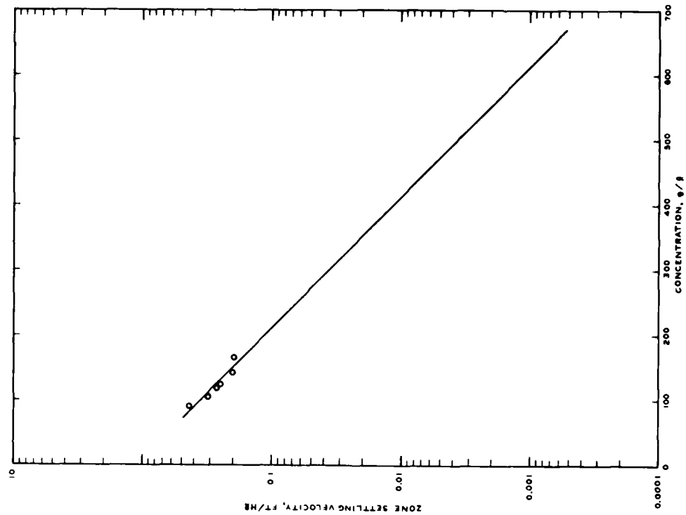
Figure 55. Zone settling velocity versus concentration, sample 1-B
