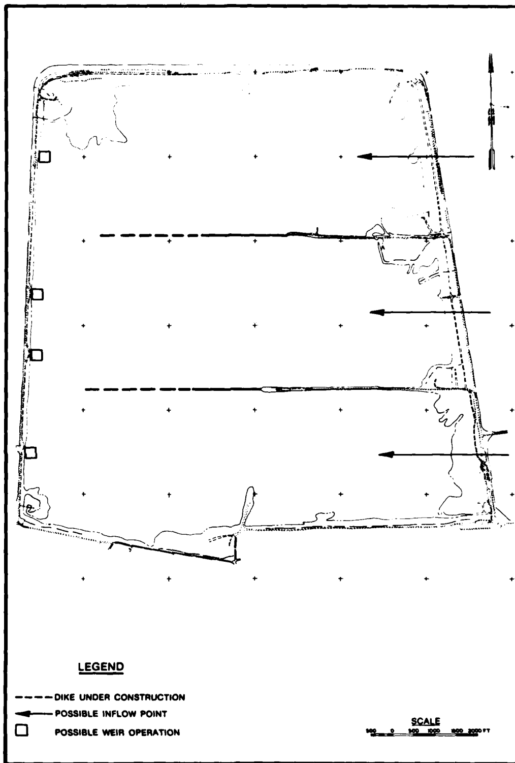
Figure 5. Stage 2 construction plan
