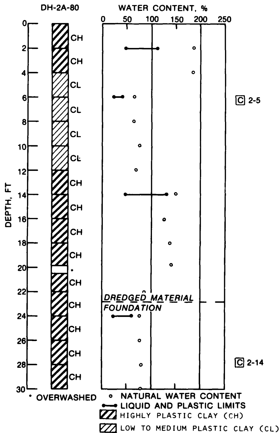
Figure 37. Boring log DH-2A-80
