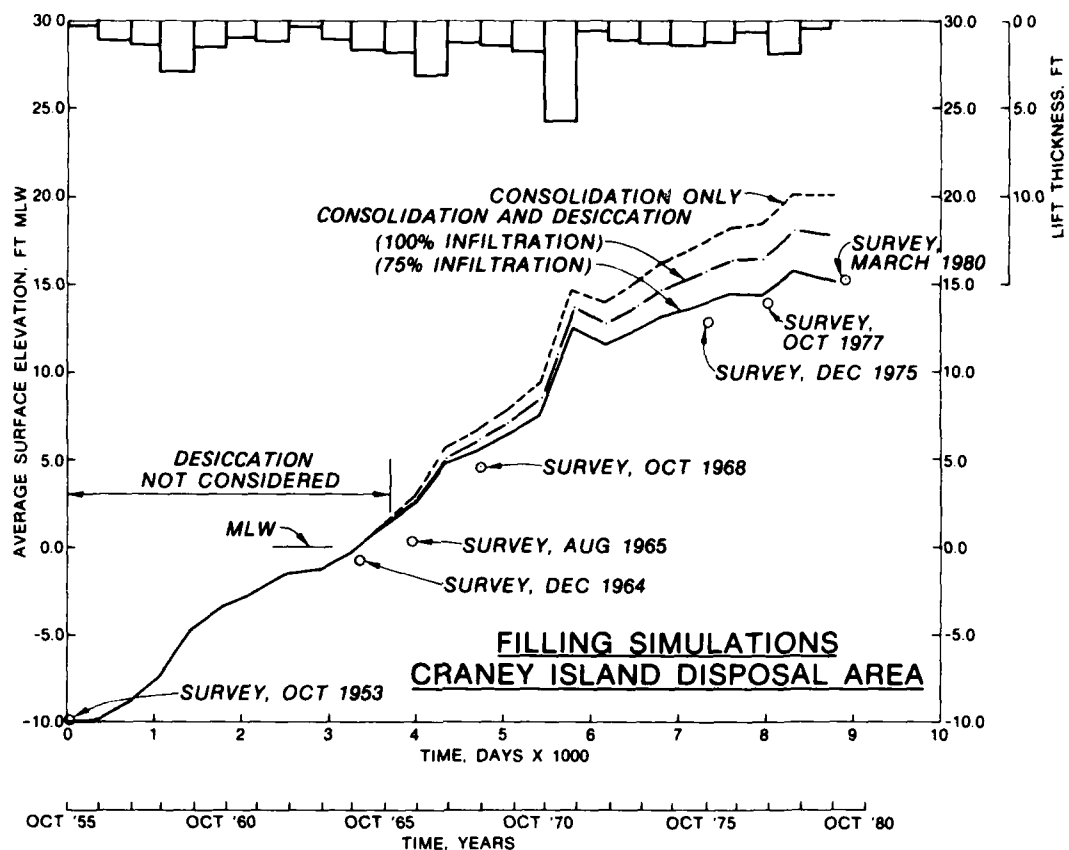
Figure 64. Simulation of filling operations 1957-1979
