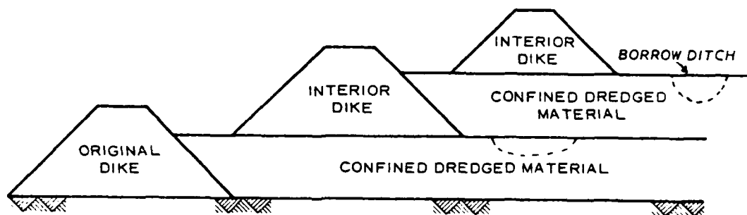
a. Concept of stepped dike construction method
