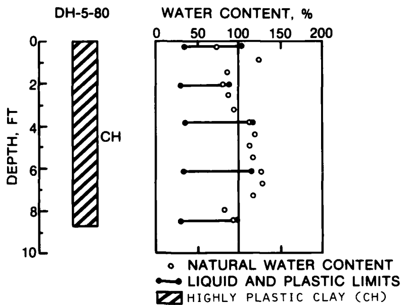
Figure 40. Boring log DH-5-80
