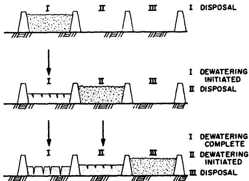
Figure 10. Concept of sequential use of subcontainments
