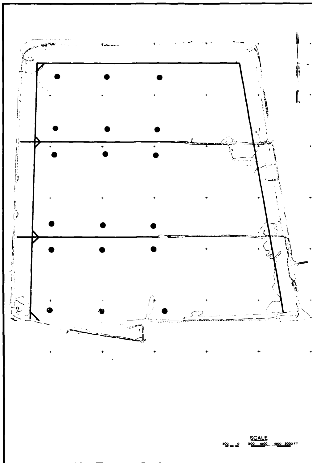
Figure 81. Suggested location of settlement plates and piezometers
