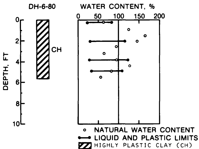
Figure 41. Boring log DH-6-80
