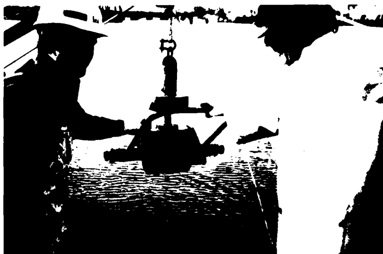
Figure 34. Shipek dredge sampler
