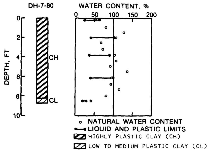
Figure 42. Boring log DH-7-80
