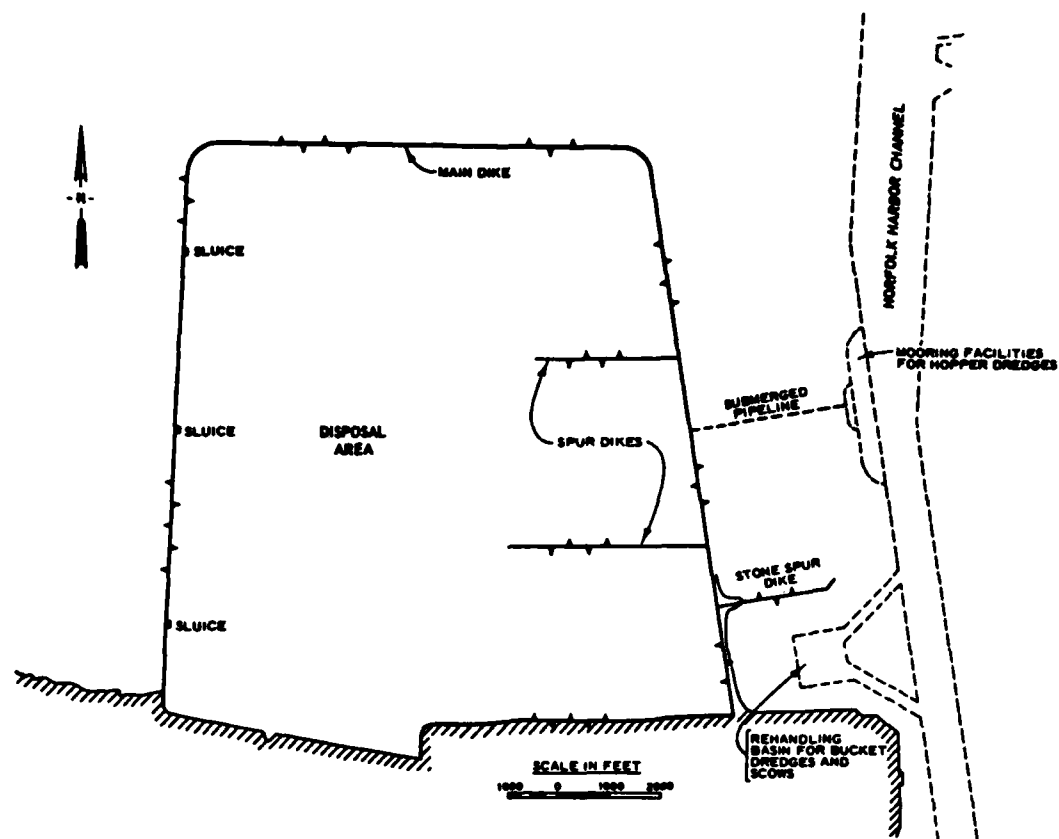
Figure 2. Layout of Craney Island disposal area
