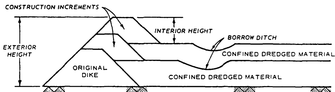
b. Concept of incremental dike construction method
