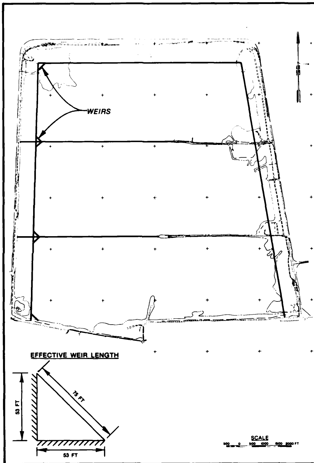
Figure 63. Recommended weir locations
