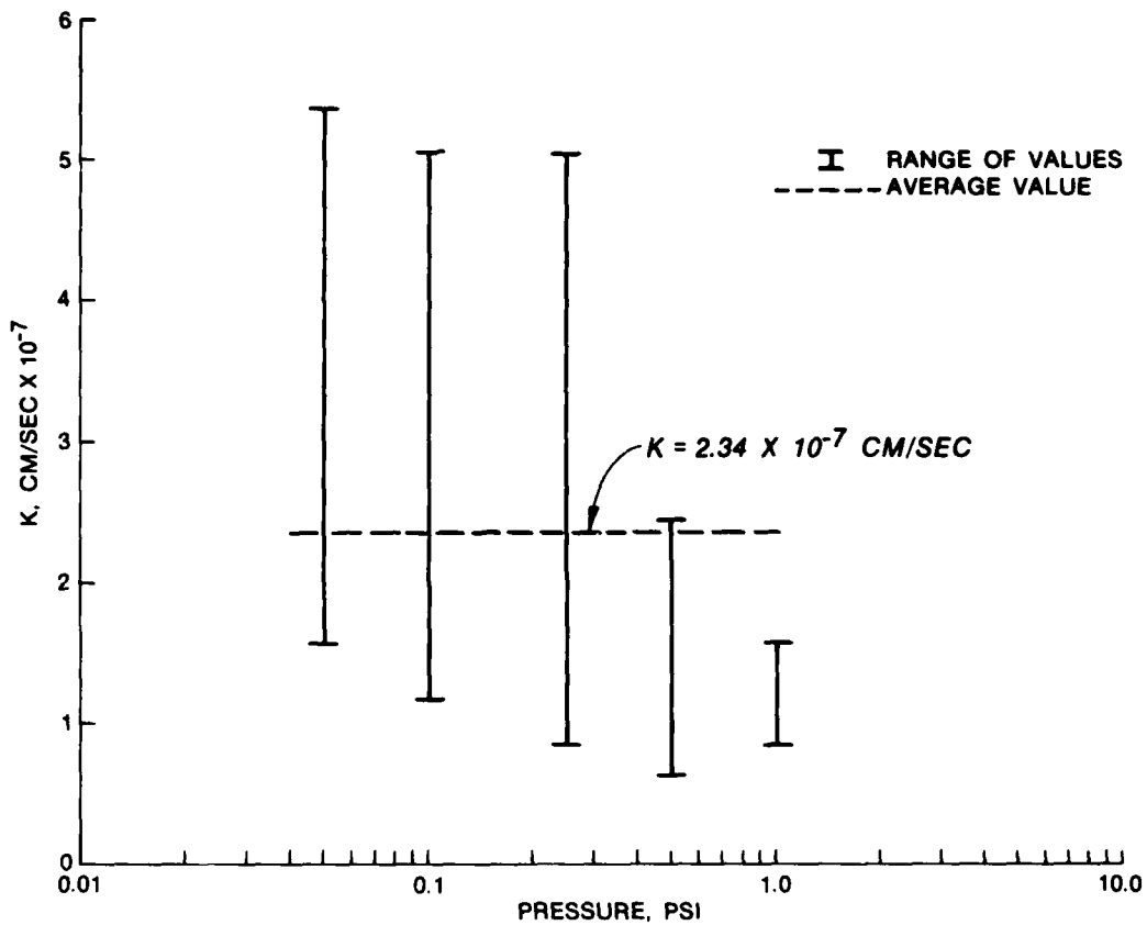
Figure 52. Coefficient of permeability versus log pressure for dredged material samples
