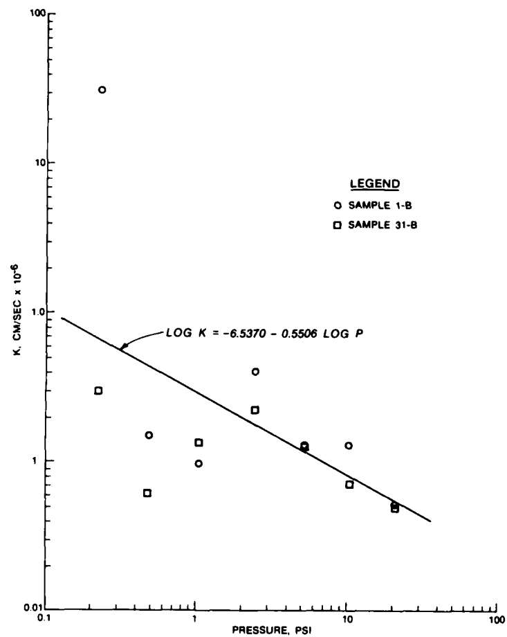
Figure 51. Coefficient of permeability versus log pressure for sediment samples
