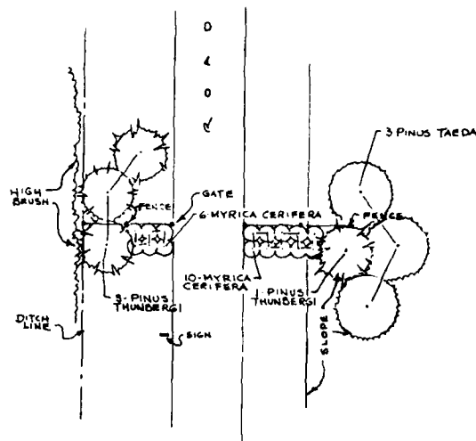
a. East gate planting plan
