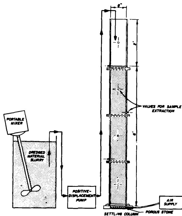
Figure 44. Sedimentation testing apparatus
