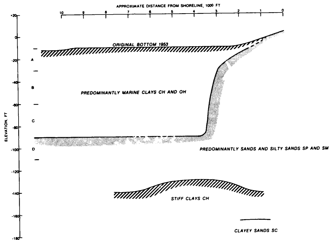
Figure 32. Generalized foundation conditions
