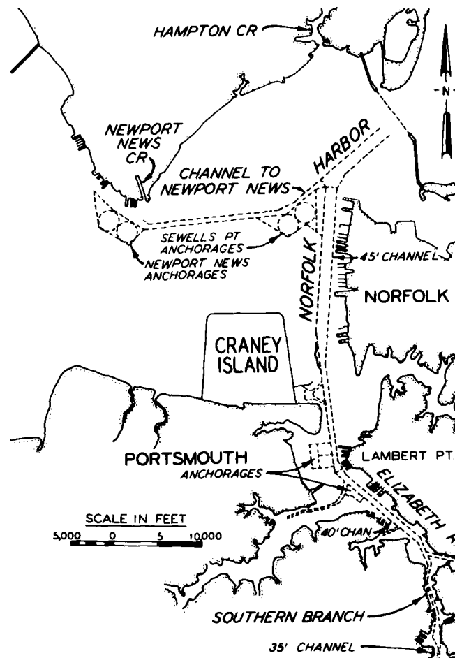
Figure 18. Channels and anchorages comprising area of Corps of Engineers maintenance responsibility
