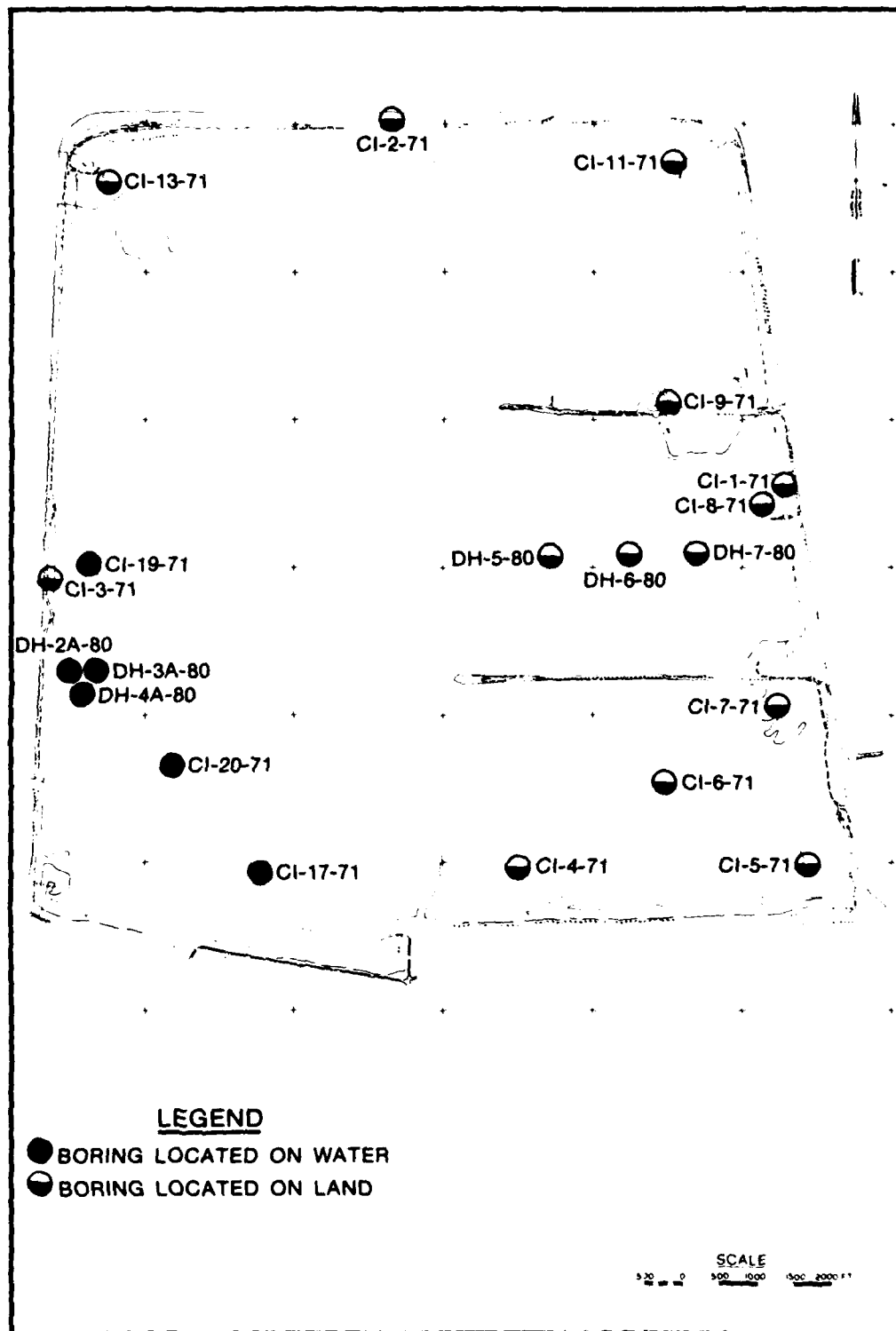
Figure 31. Boring plan
