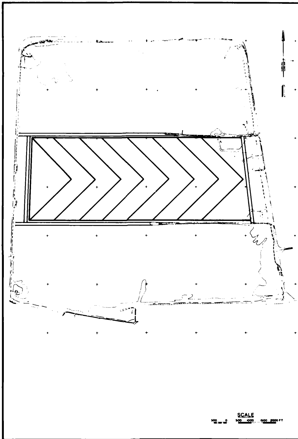
Figure 13. Interior trench layout for dredged material dewatering
