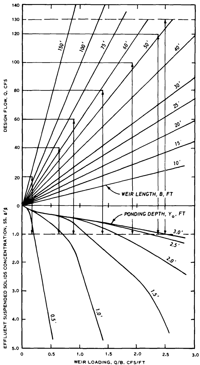
Figure 62. Nomogram relating weir design parameters (after Walski and Schroeder 1978)
