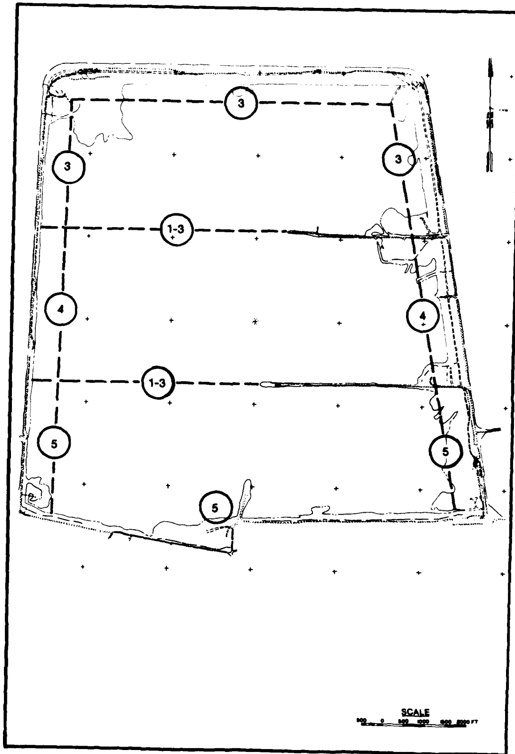
Figure 79. Dike construction sequence
