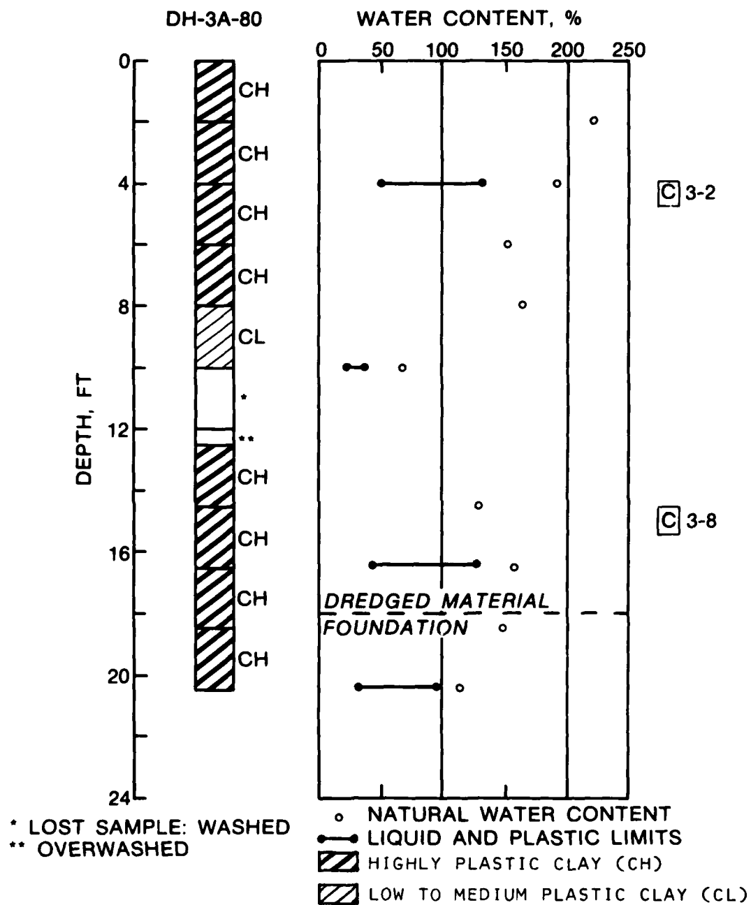
Figure 38. Boring log DH-3A-80
