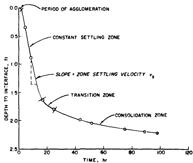
Figure 45. Typical zone settling test results
