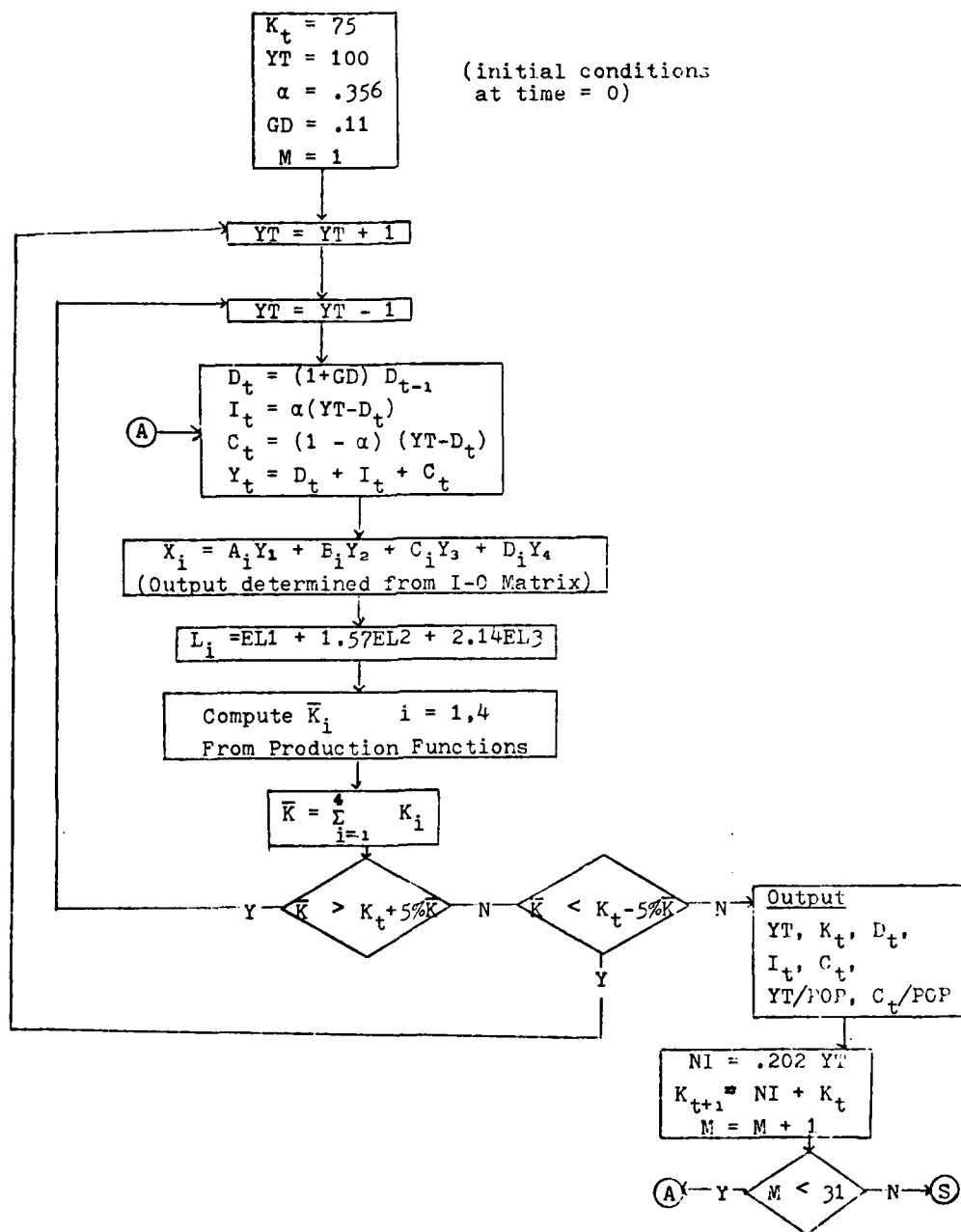
Figure 9. Growth Model
