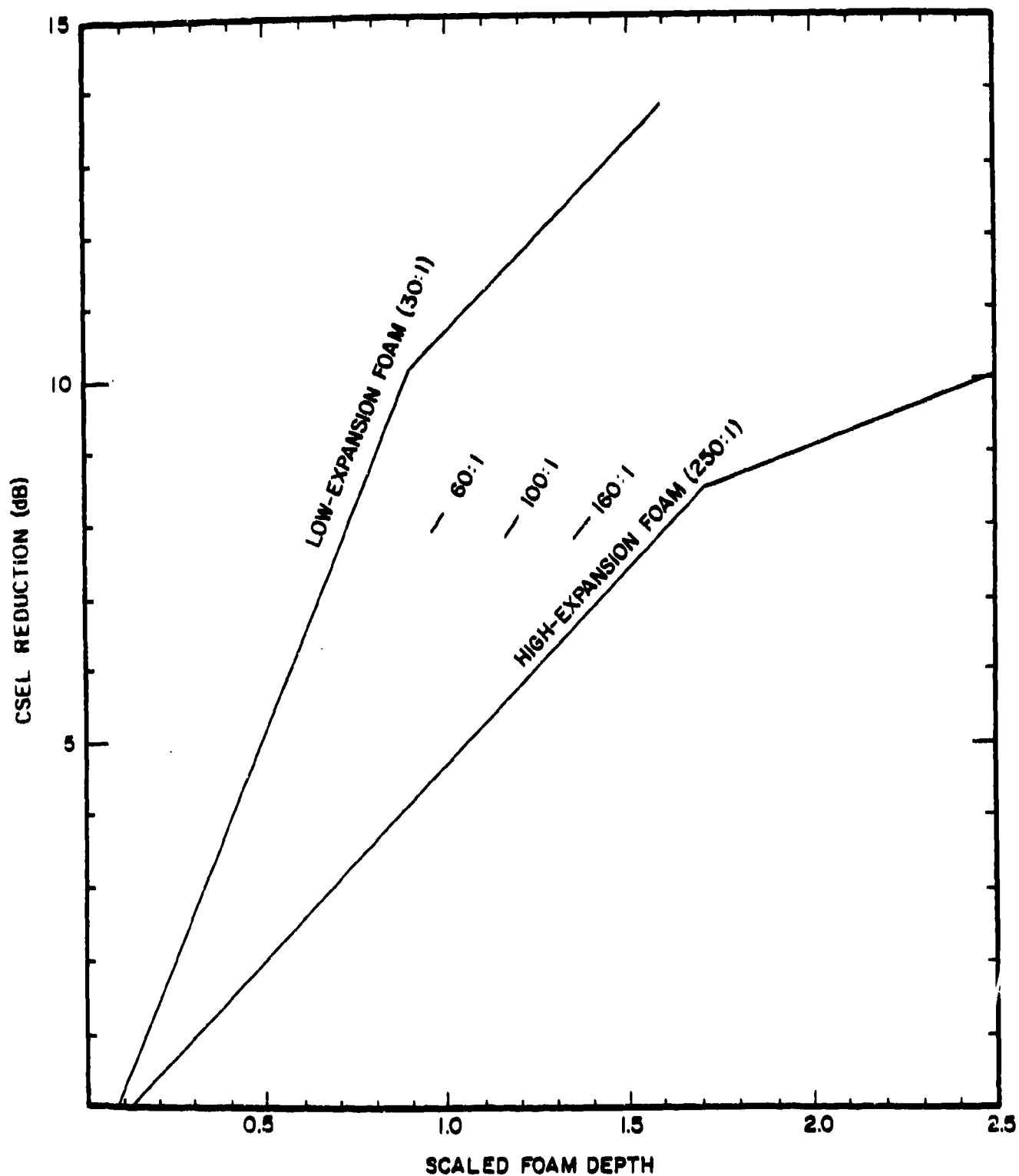
Figure 21. CSEL reduction prediction curves.
