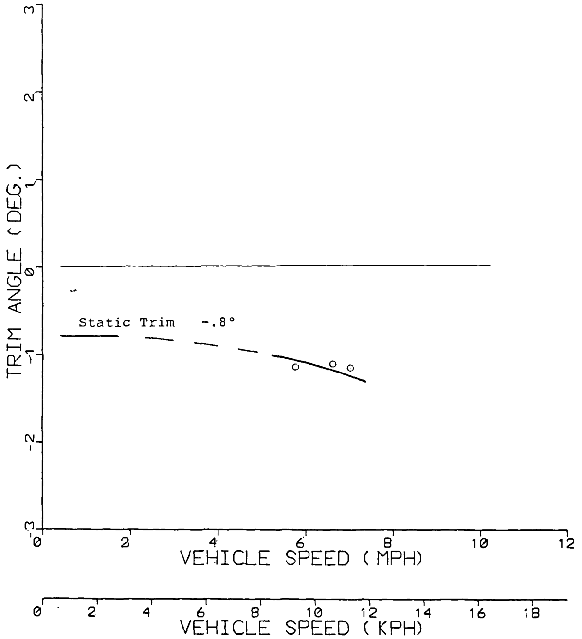
FIGURE 11. Trim Angle (Deg.) as a Function of the Vehicle Speed for the Single "Y15" Without Bow Plane Initial Static Trim -0.8^\circ
