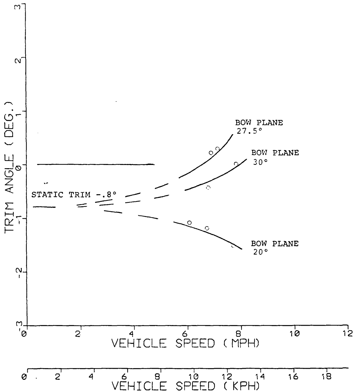
FIGURE 12. Trim Angle (Deg.) as a Function of the Vehicle Speed for Single "Y15" With Large Bow Plane at 3 Different Bow Plane Angles of Attack (20°, 27.5°, 30°) Initial Static Trim -0.8°
