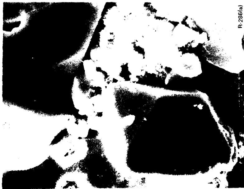
Fig. 21 — Positive active material at the end of cycle 1 discharge at 18 \text{ A/m}^2 , the 24-hr rate. The smallest particles are \text{PbO}_2 . Medium size and large crystals are \text{PbSO}_4 . Magnification 5000X.
