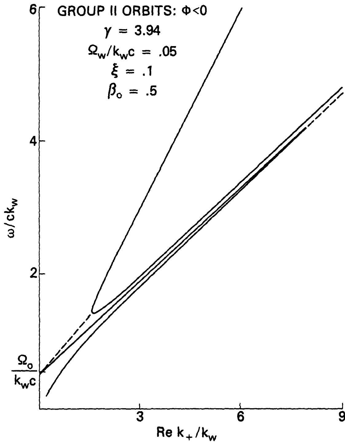
Fig. 8 — Graph of \omega/ck_w versus \text{Re } k_+ / k_w for group II orbits ( \Phi < 0 ) and \beta_o = .5
