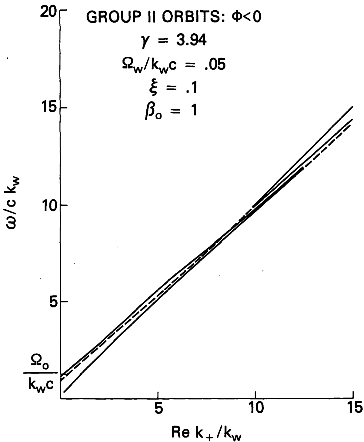
Fig. 10 — Graph of \omega/c k_w versus \text{Re } k_+ / k_w for group II ( \Phi < 0 ) orbits and \beta_0 = 1
