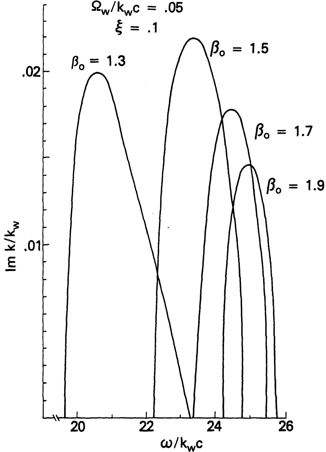
Fig. 6 — Graph of \text{Im } k/k_w versus \omega/k_w c for group II orbits ( \Phi > 0 )
