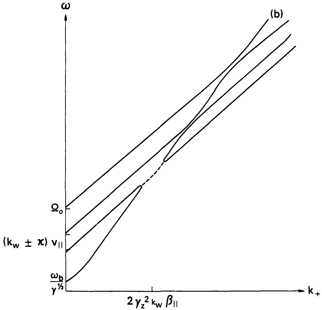
Fig. 4 (Continued) — Schematic representation of the interaction for group I (a) and group II (b) orbits when \Phi > 0 . The dotted line denotes complex conjugate roots.
