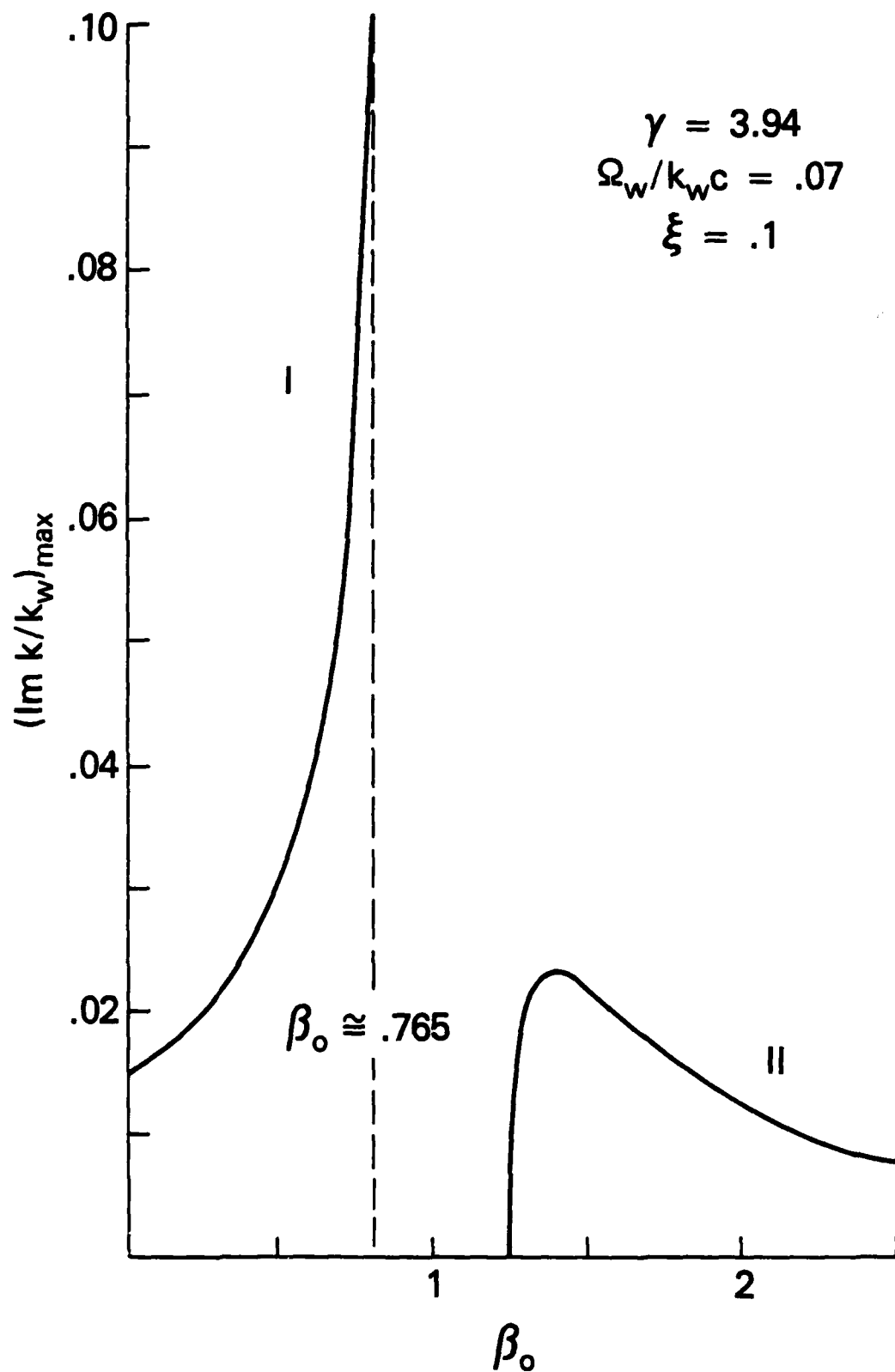
Fig. 7 - Graph of (\text{Im } k/k_w)_{\text{max}} as a function of the axial guide field for group I and II ( \beta > 0 ) orbits
