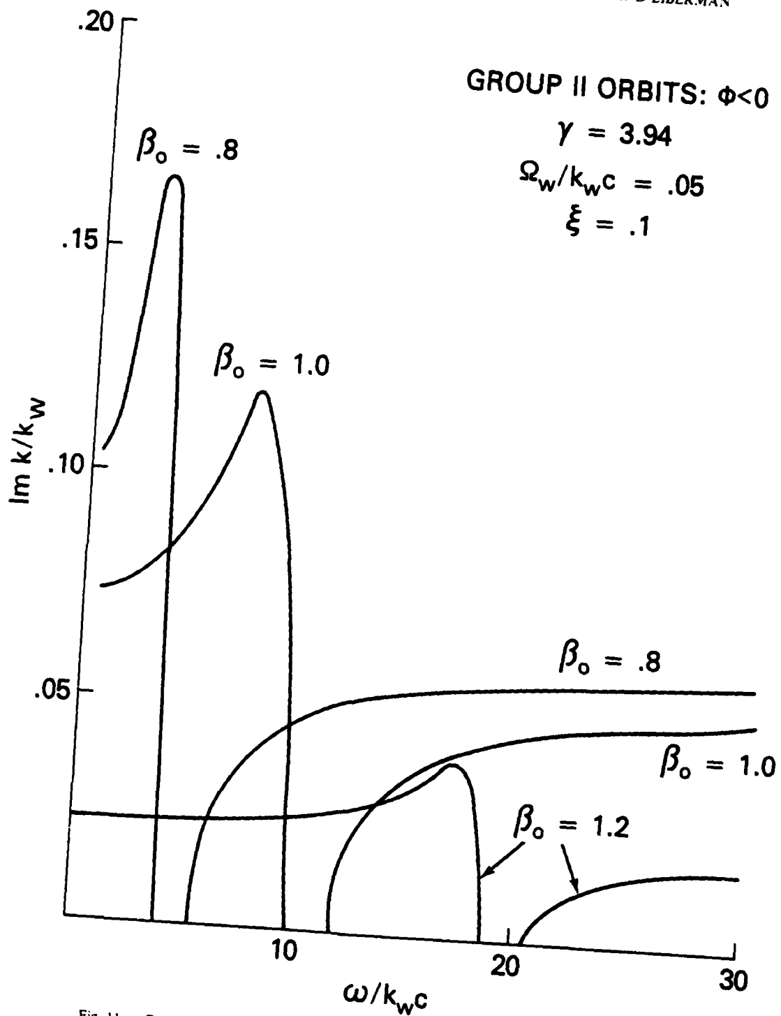
Fig. 11 — Graph of \text{Im } k/k_w versus \omega/k_w c for group II ( \phi < 0 ) orbits and \beta_0 = .8, 1, and 1.2
