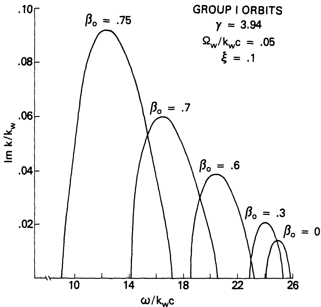
Fig. 5 — Graph of \text{Im } k/k_w versus \omega/k_w c for group I orbits
