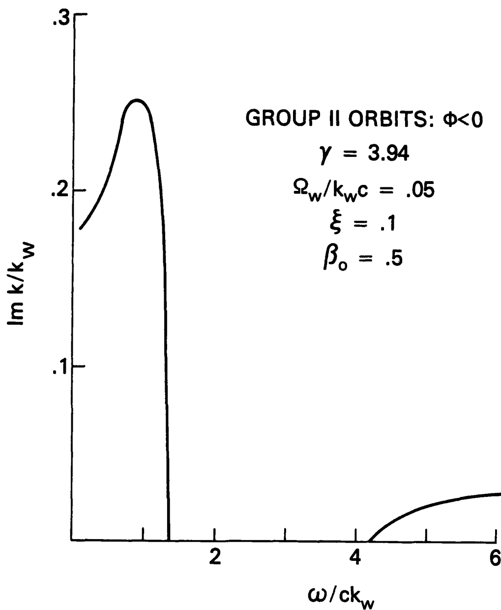
Fig. 9 — Graph of \text{Im } k/k_w versus \omega/ck_w for group II ( \Phi < 0 ) orbits and \beta_0 = .5
