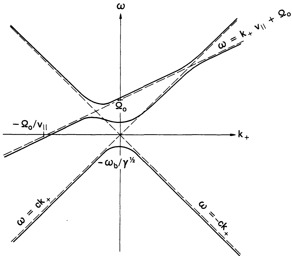
Fig. 2 — Schematic representation of the dispersion curves for the \delta A_+ mode showing the passive interaction between the cyclotron and the pure electromagnetic mode at \omega \approx (1 - \beta^2)^{-1}\Omega_0
