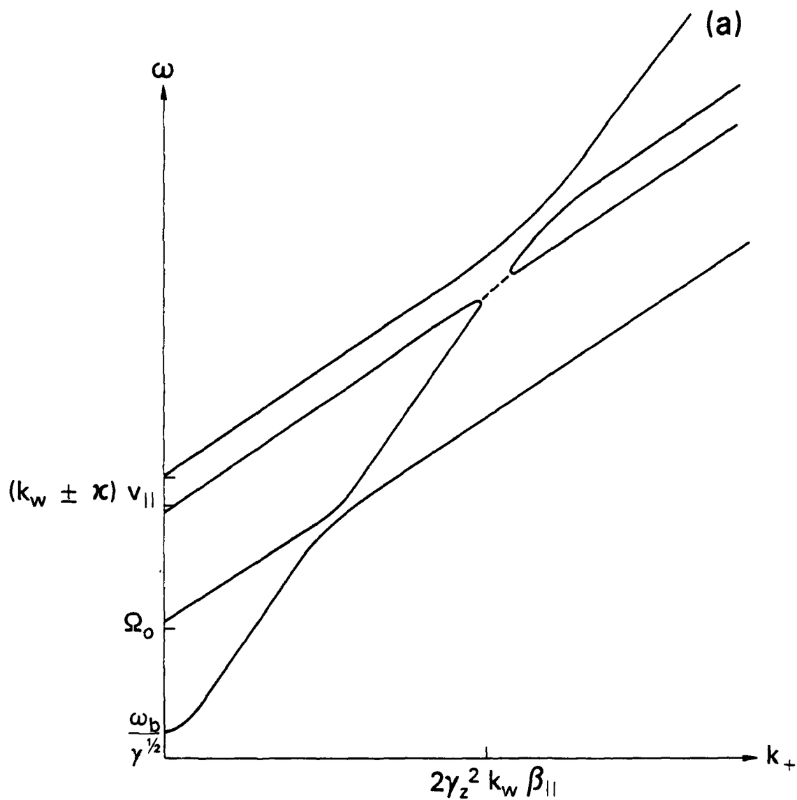
Fig. 4 — Schematic representation of the interaction for group I (a) and group II (b) orbits when \Phi > 0 . The dotted line denotes complex conjugate roots.
