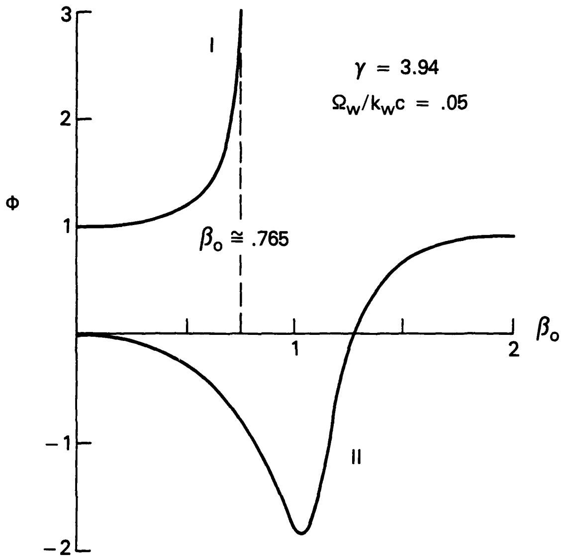
Fig. 3 — Graph of \Phi versus \beta_0 for both group I and group II orbits for a beam energy of 1.5 MeV and a wiggler amplitude and period such that \Omega_w/k_wc = .05
