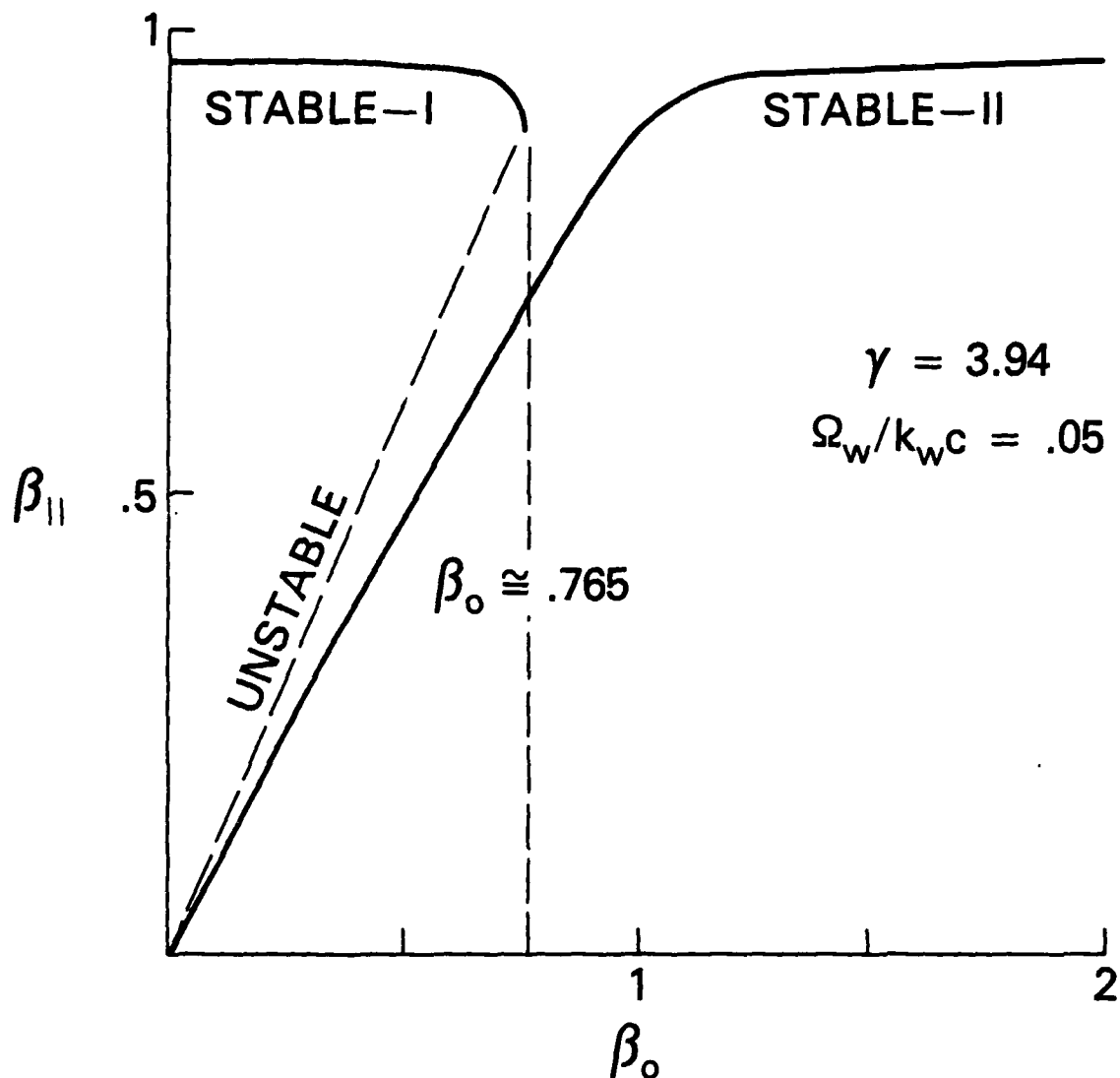
Fig. 1 — Graph of the axial velocity versus \beta_0 ( \equiv \Omega_w/k_wc ) for a beam energy of 1.5 MeV and a wiggler amplitude and period such that \Omega_w/k_wc = .05
