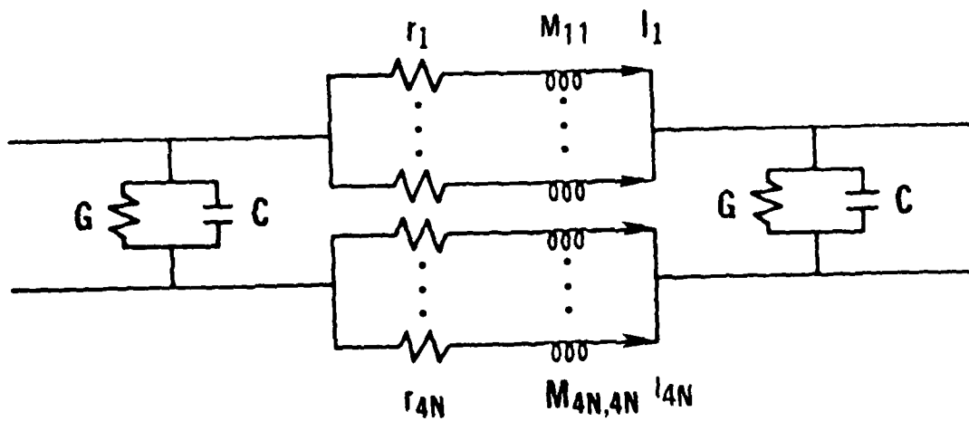
Figure 3. Equivalent circuit.
