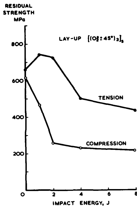
Fig 19 Residual tensile and compressive strengths of CFRP showing effect of delamination at low impact energies and flexural failure of 0° fibres at higher energies (G. Dorey, D.J. Portsmouth)
