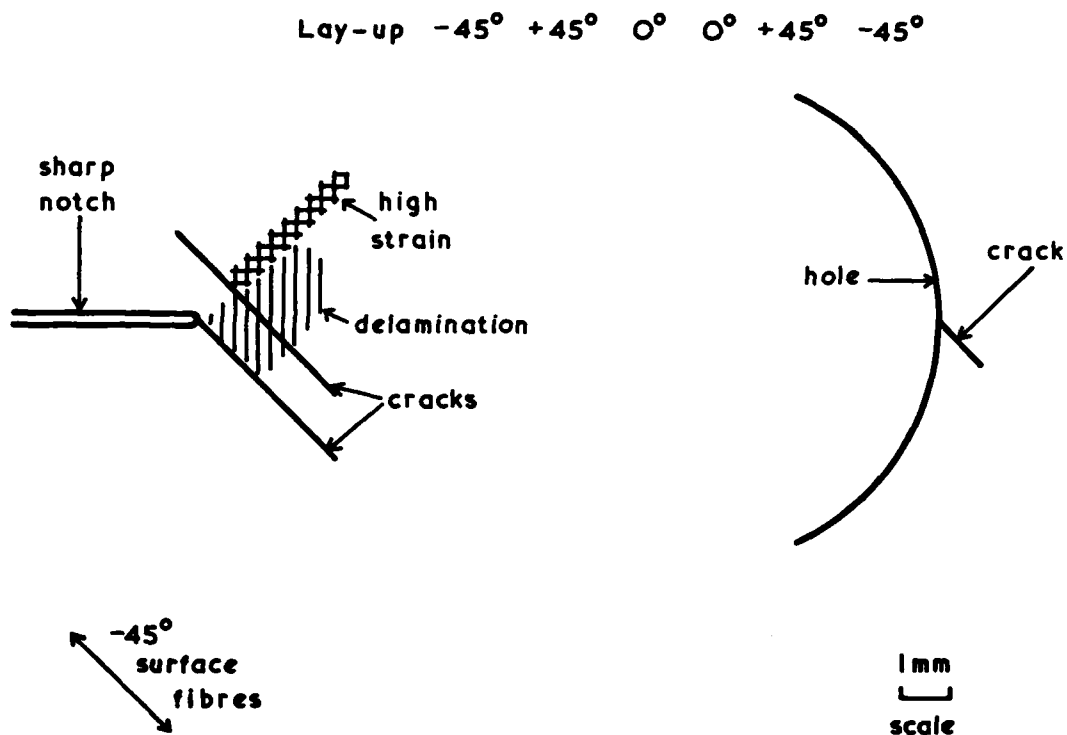
Fig 12 Damage zones at a sharp notch and a circular hole in CFRP under tension (S.M. Bishop)
