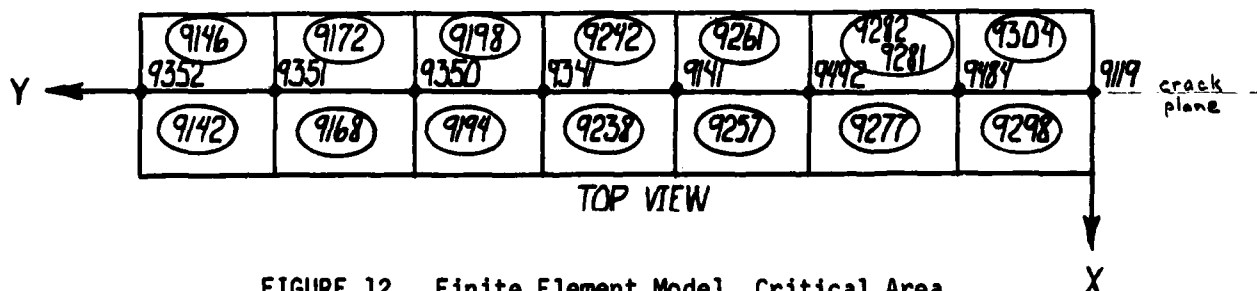
FIGURE 12. Finite Element Model, Critical Area Elements
