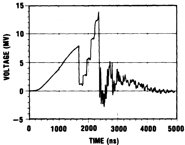
(c) TRANSFER SWITCH, S 1 (MARX SIDE)
