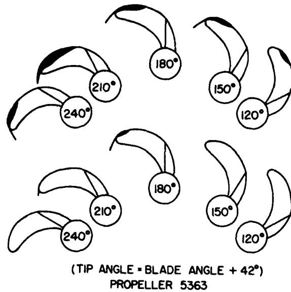
FIG. 13: CALCULATED AND MEASURED SUCTION-SIDE CAVITATION PATTERNS, PROPELLER 5363.
