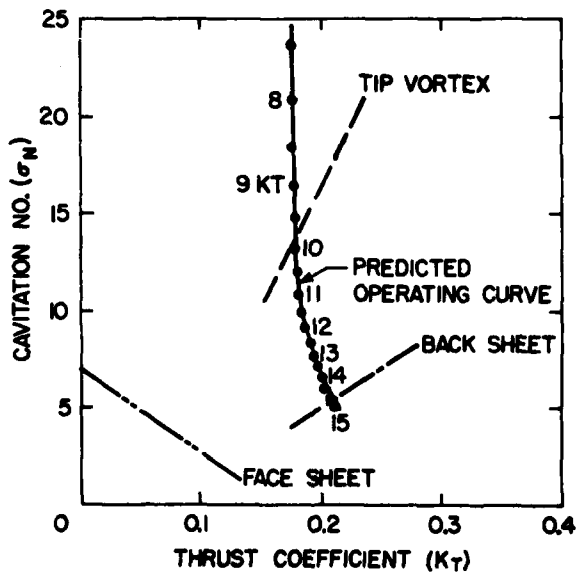
FIG. 10: CAVITATION INCEPTION, PROPELLER 5363, BEHIND CONDITION. DRAUGHT, 4650 MM.
