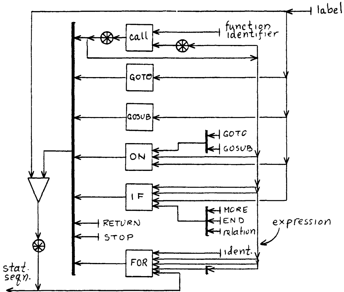
Figure 16. BASIC Control Structures
