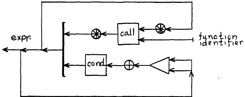
Figure 14. LISP Control Structures
