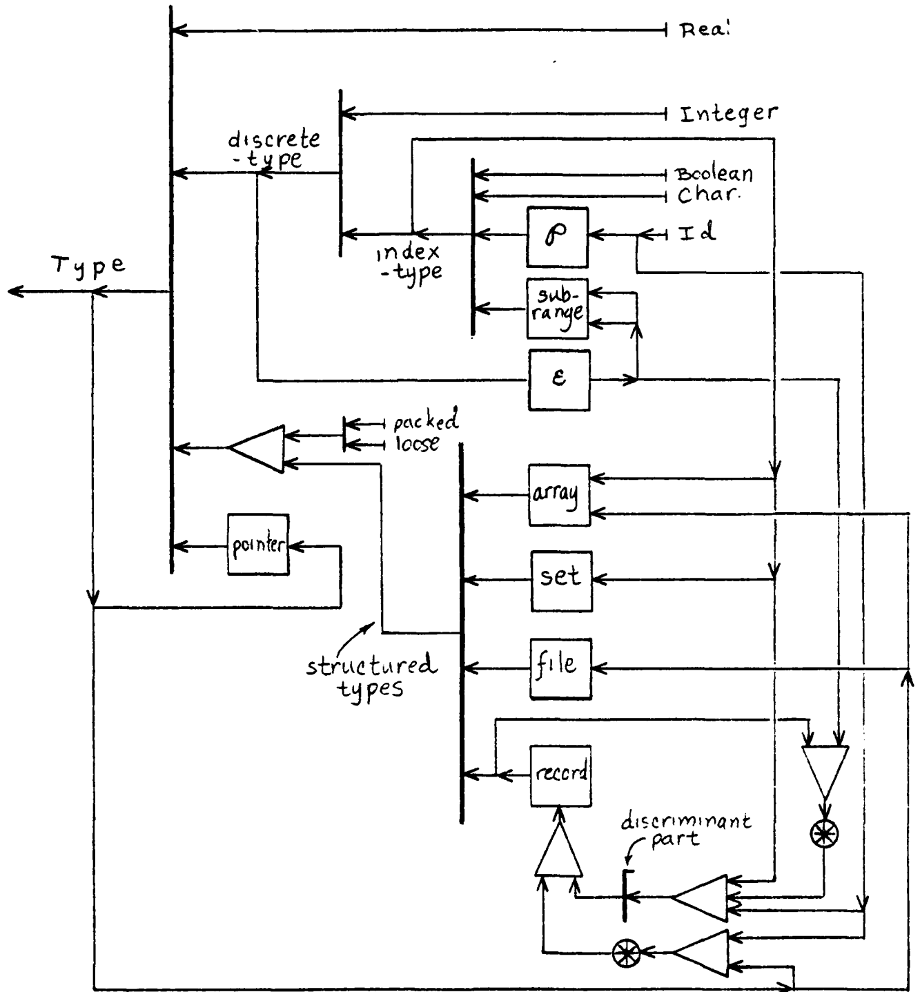
Figure 2. The Pascal Type System
