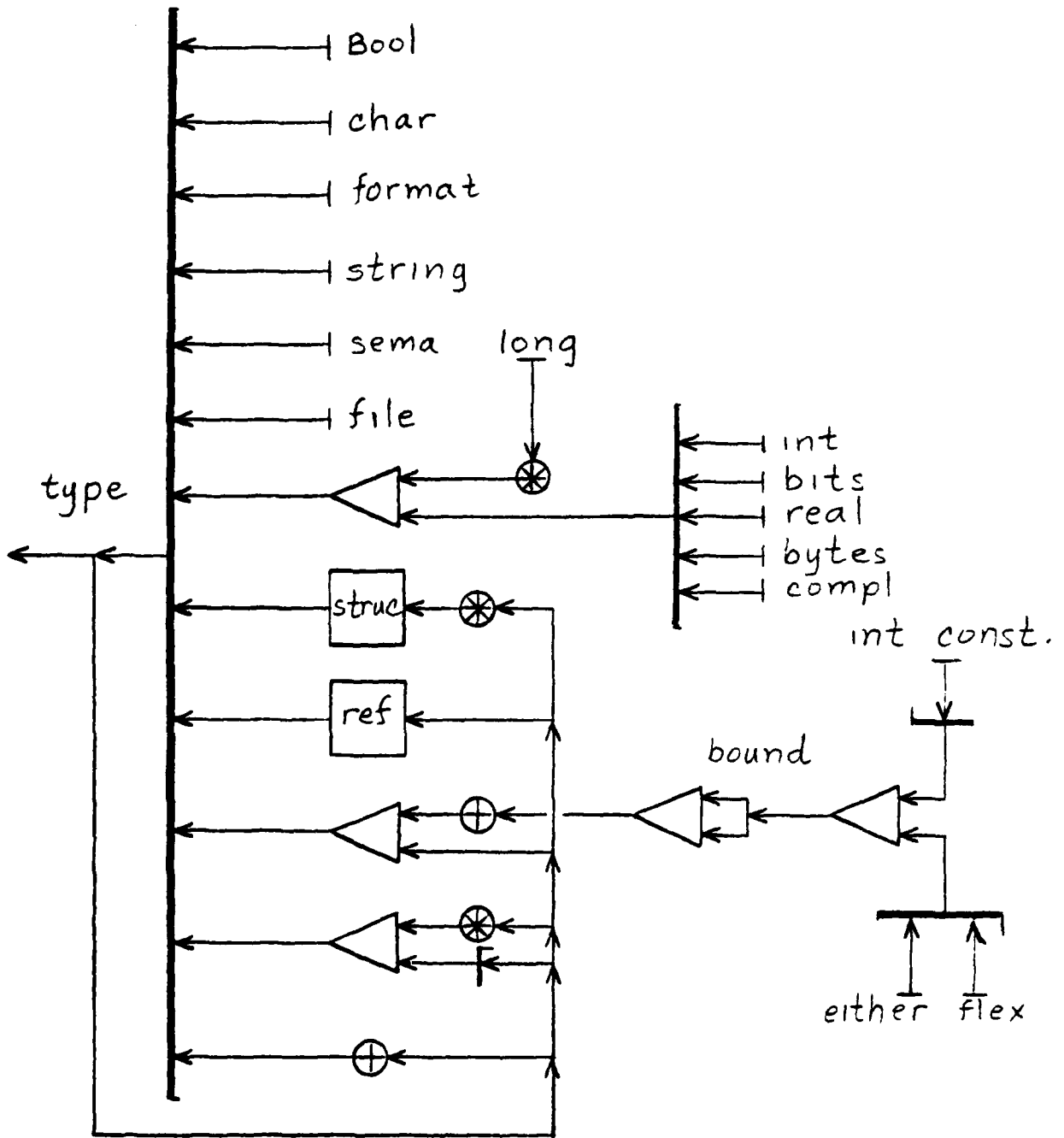
Figure 5. The Algol-68 Type System
