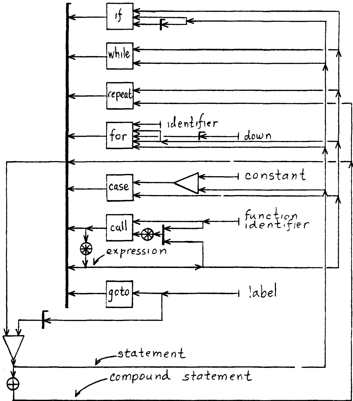
Figure 13. Pascal Control Structures
