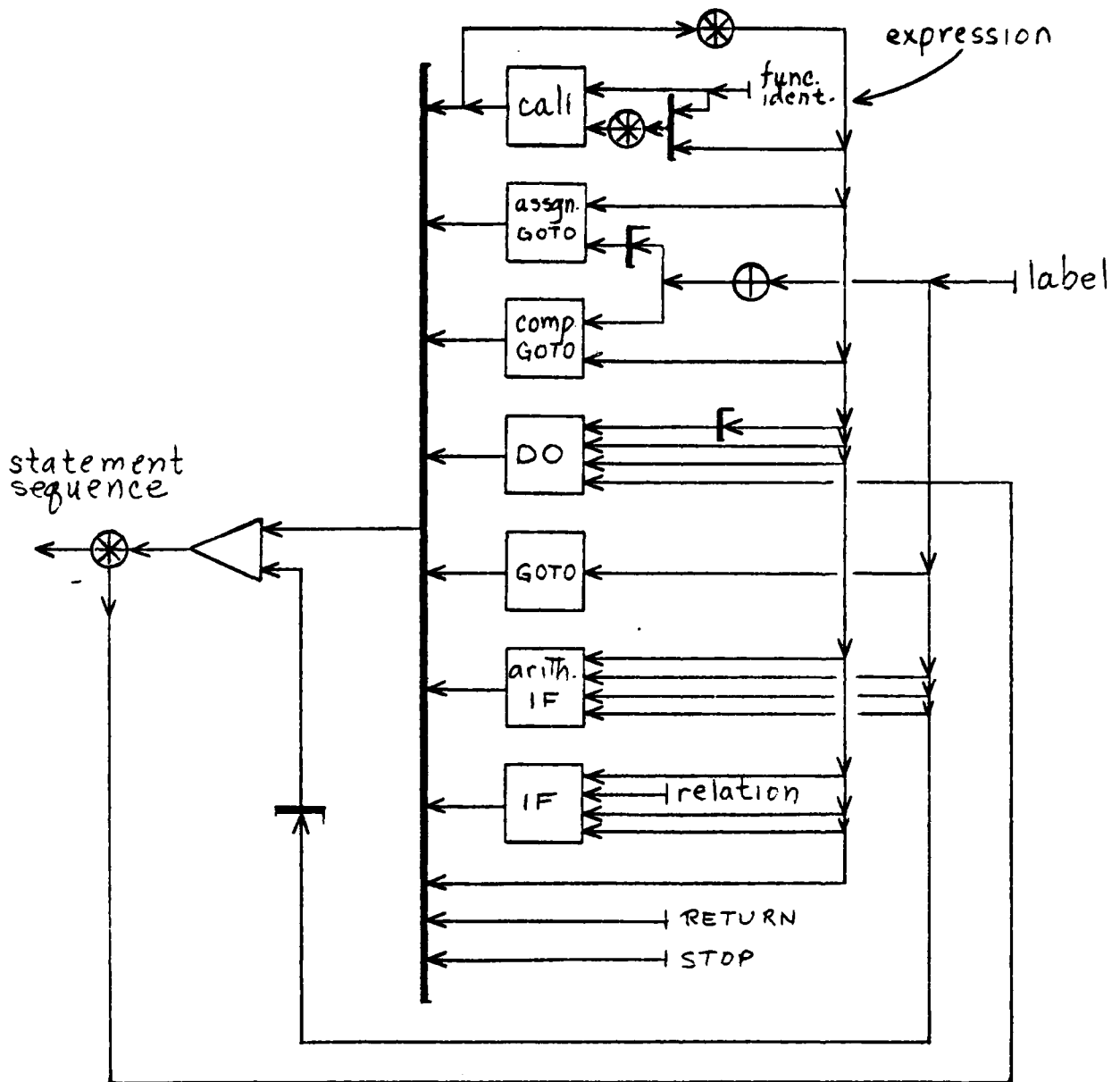
Figure 15. FORTRAN Control Structures
