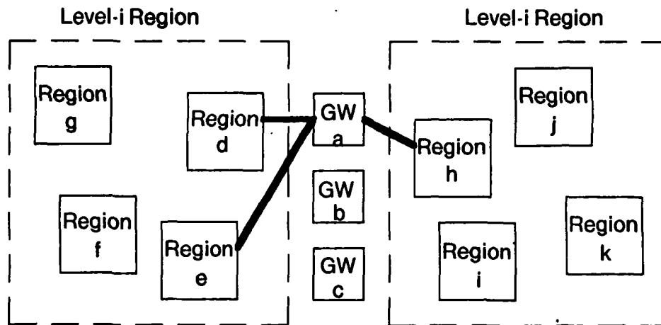
Figure 3-7: Increasing or decreasing a level-i region
