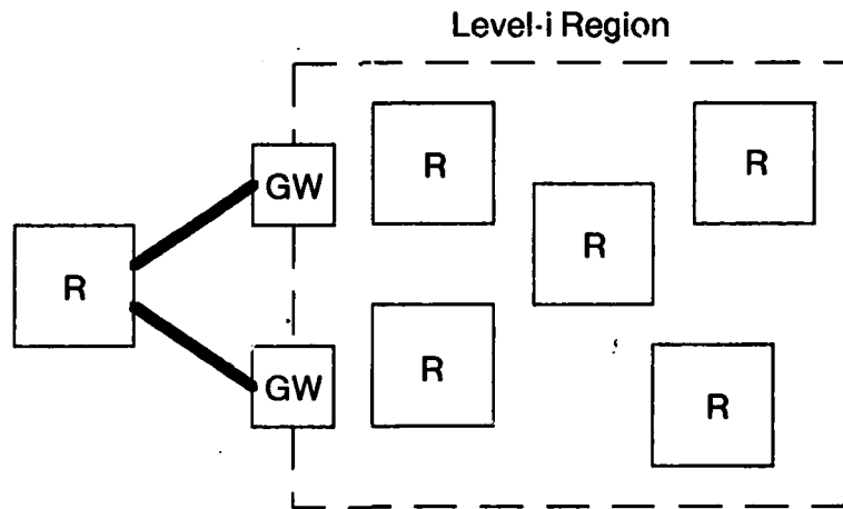
Figure 3-5: Adding or taking away a level-( i - 1 ) region
