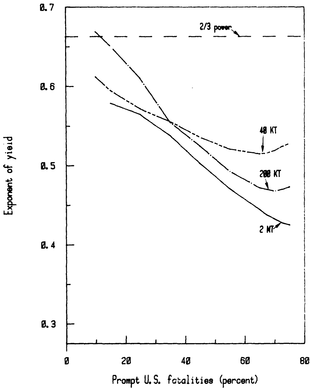
Fig. 12--Exponent of yield required to produce true "equivalent megatons" for various Soviet yields used to attack U.S. population
