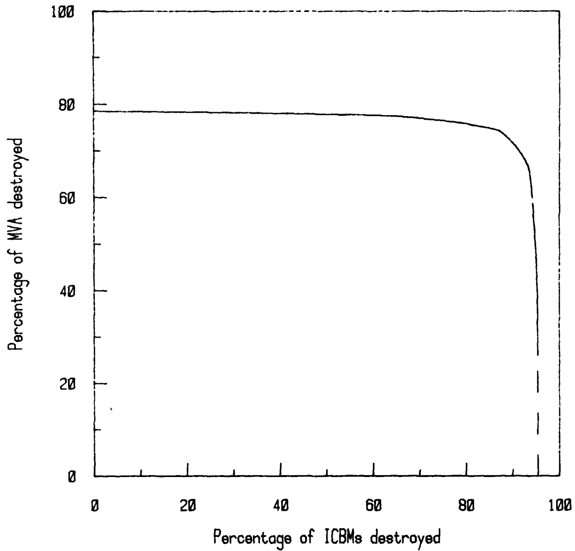
Fig. 16--Exemplary tradeoff between counterforce and countervalue damage
