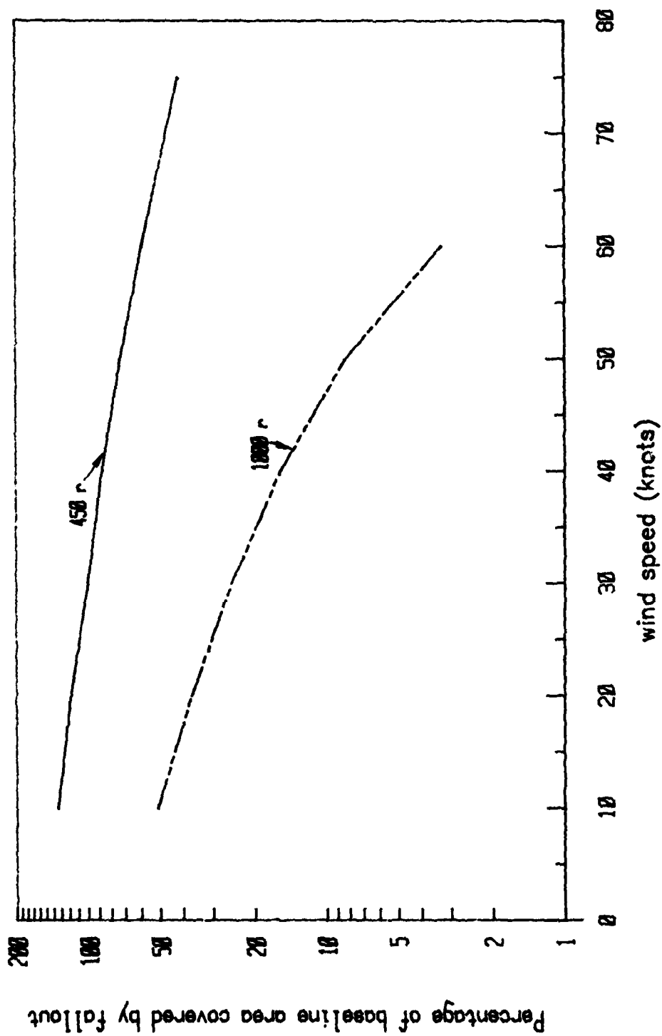
Fig. 10--Impact of wind speed on the lethal area covered by a single fallout pattern
