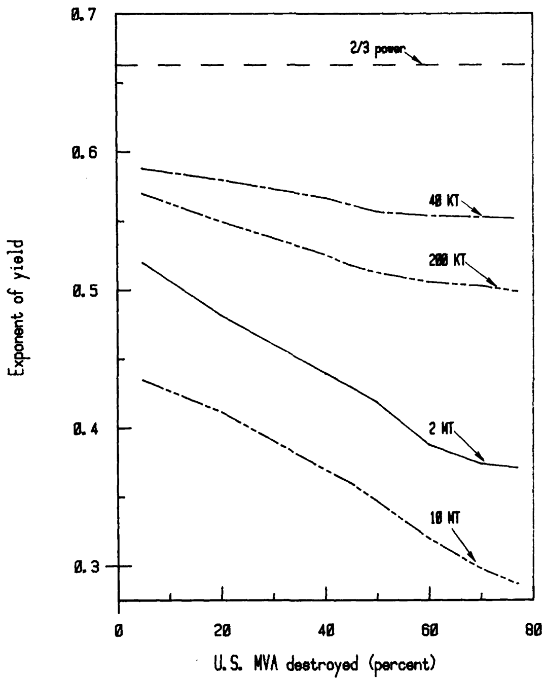
Fig. 11--Exponent of yield required to produce true "equivalent megatons" for various Soviet yields used to attack U.S. industry
