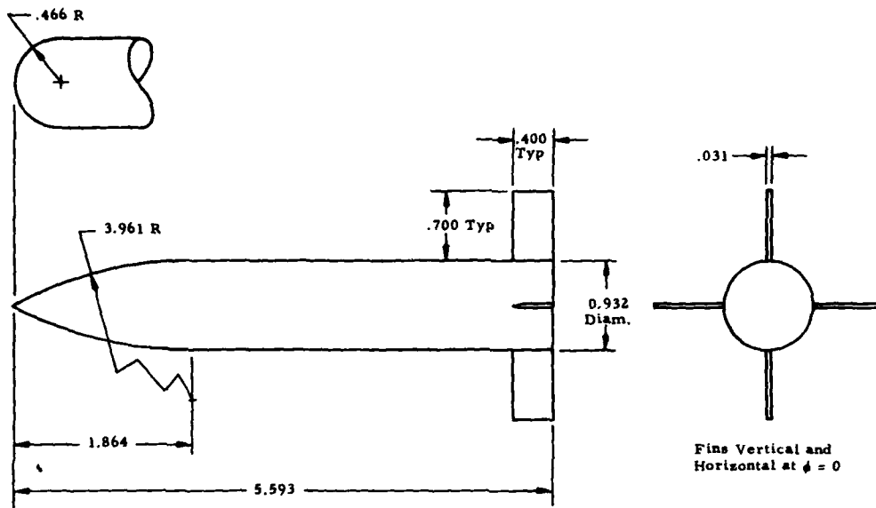
Figure 1. Submissile Design
