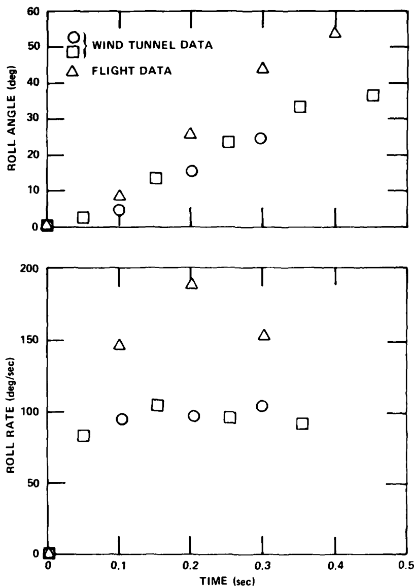
Figure 4 - Roll Motion
