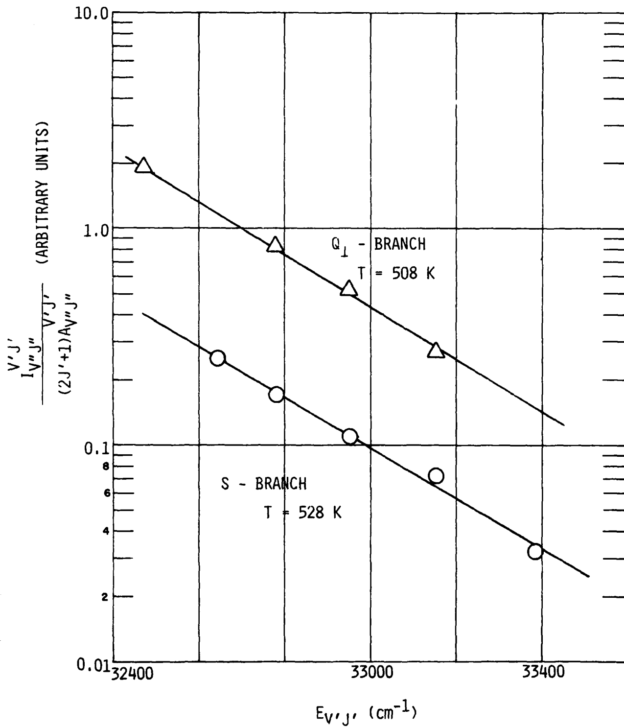
Fig. 4 Maxwell-Boltzmann rotational plot for a 50 watt lamp in 2 torr Ar and 7 mtorr \text{H}_2\text{O} .
