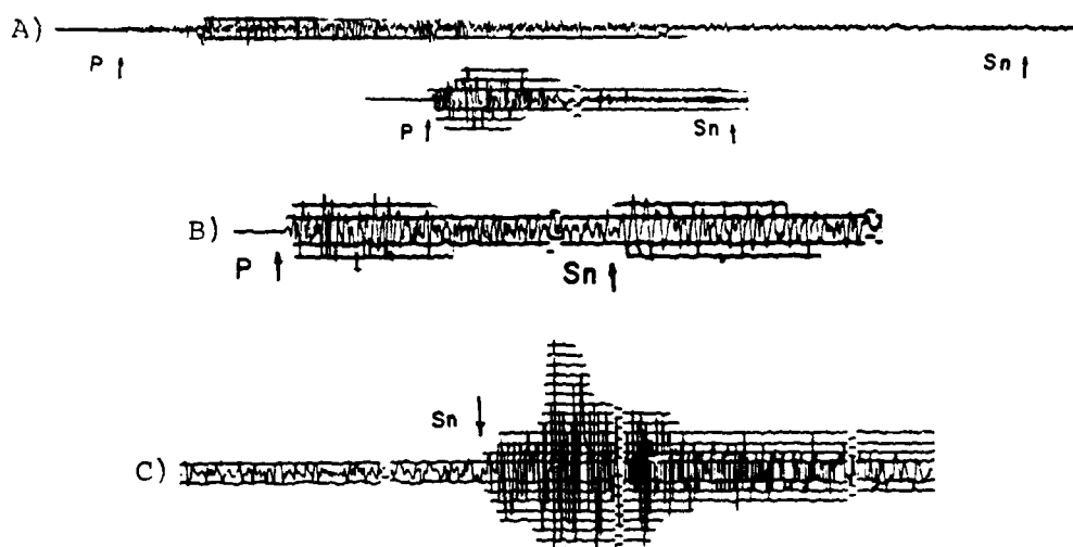
Figure 8. Examples of S_n phases observed along paths with varying efficiency of propagation. From the top to bottom: A) Inefficient propagation with S_n missing. B) More efficient propagation with S_n having about the same amplitudes as P and showing predominantly low-frequency characteristics. C) Efficient propagation with a large high-frequency S_n (after Molnar and Oliver, 1969).
