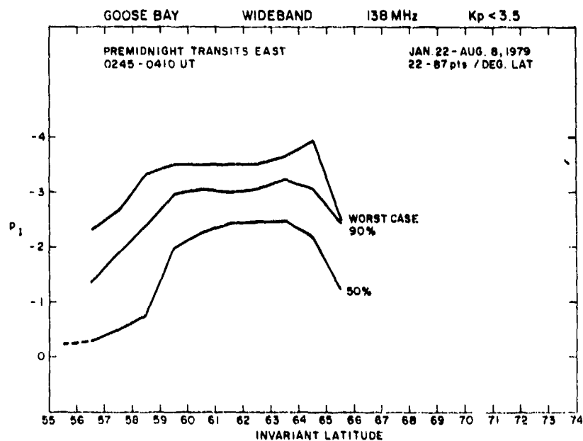
Figure 25a. Intensity Spectral Index p_1 vs. Invariant Latitude for Nighttime Transits East of Goose Bay Under Quiet Magnetic Conditions
