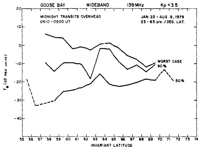
Figure 14a. Spectral Strength T_\phi of Phase at 1 Hz vs. Invariant Latitude for Nighttime Transits Overhead of Goose Bay Under Quiet Magnetic Conditions
