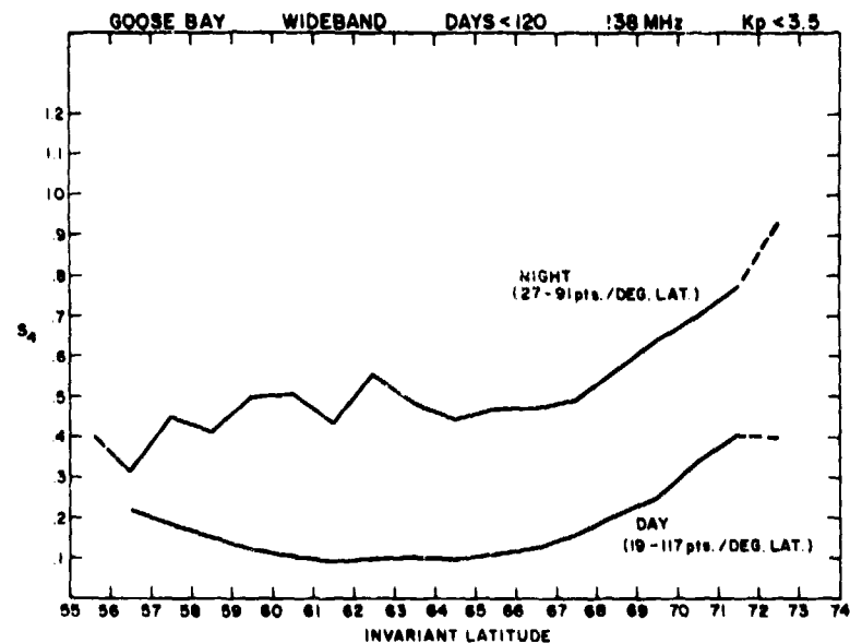
Figure 82. Amplitude Scintillation Index S_4 Observed During the Vernal Equinox (22 January through 30 April 1979) at Goose Bay as a Function of Invariant Latitude Under Quiet Magnetic Conditions ( K_p < 3.5 ) Separated into Night and Daytime Periods
