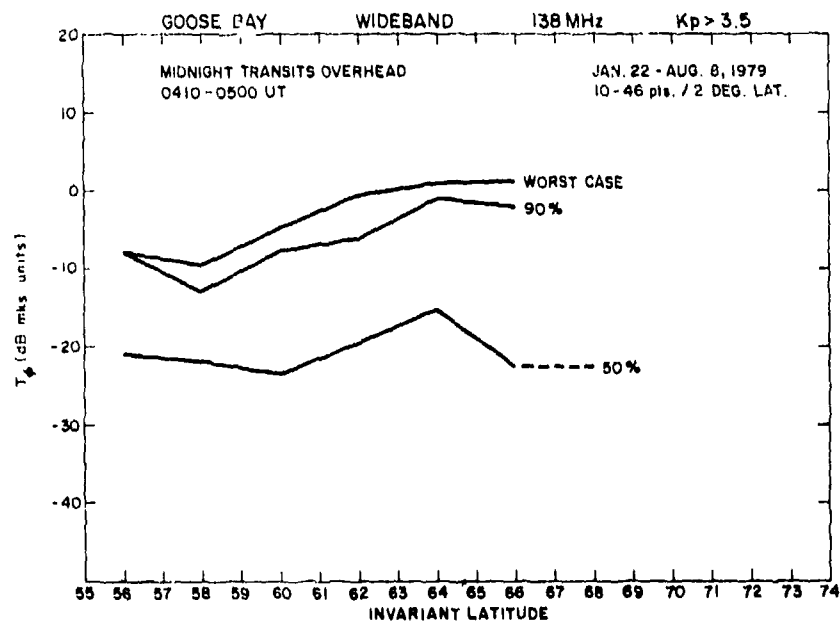
Figure 14b. Spectral Strength T_\phi of Phase at 1 Hz vs. Invariant Latitude for Nighttime Transits Overhead of Goose Bay Under Disturbed Magnetic Conditions
