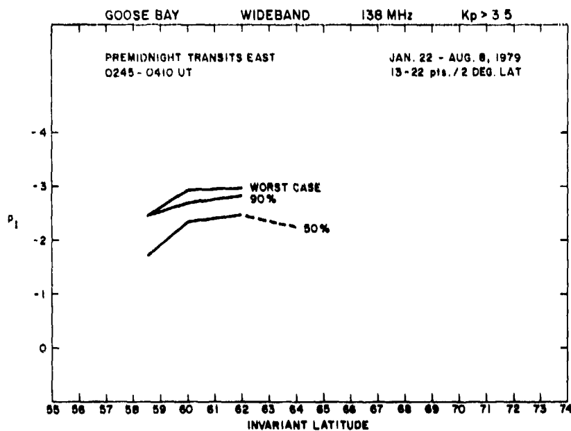
Figure 25b. Intensity Spectral Index p_1 vs. Invariant Latitude for Nighttime Transits East of Goose Bay Under Disturbed Magnetic Conditions
