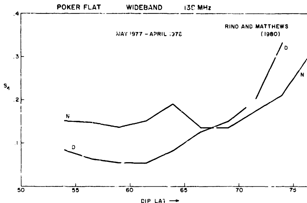
Figure 86. Amplitude Scintillation Index S_4 at Poker Flat During 1977-1978 as a Function of Dip Latitude Separated into Day and Nighttime Periods (Rino and Matthews, 1980) c
