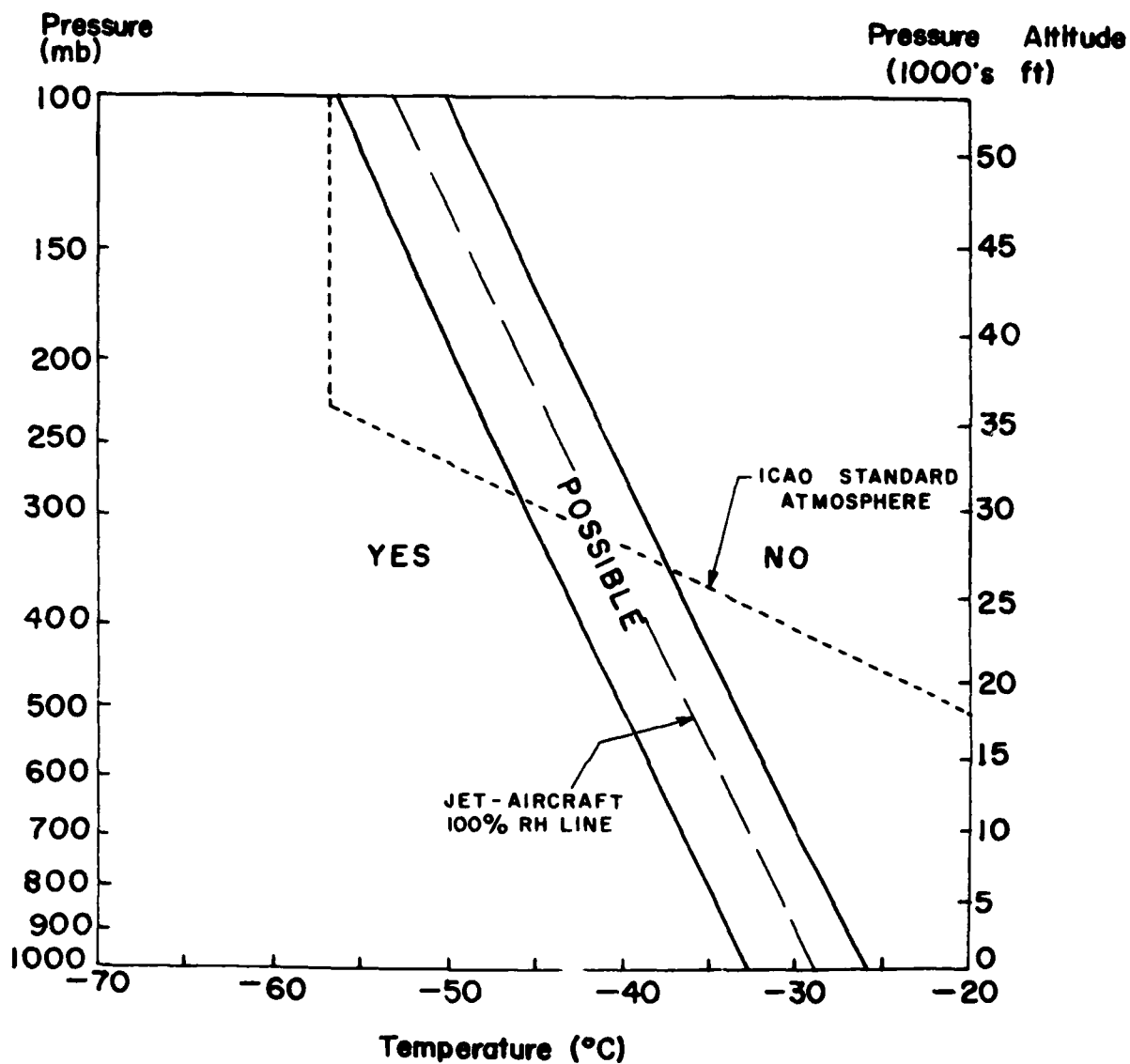
Figure 4. Propeller Aircraft Contrail-Formation Graph.
