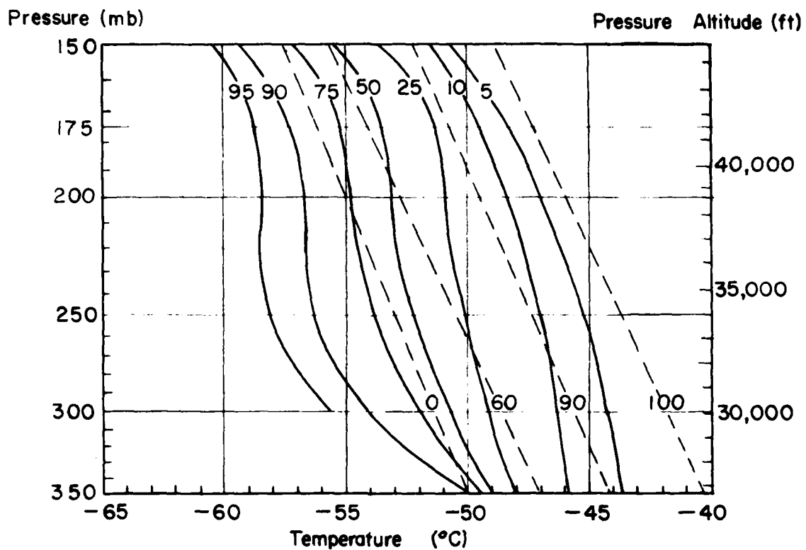
Figure 3. Probability of Jet Aircraft Contrail Formation as a Function of Pressure and Temperature. Solid lines are empirically derived curves of contrail probability (percent). Dashed lines are theoretically derived curves of minimum relative humidity (percent) required for contrail formation.
