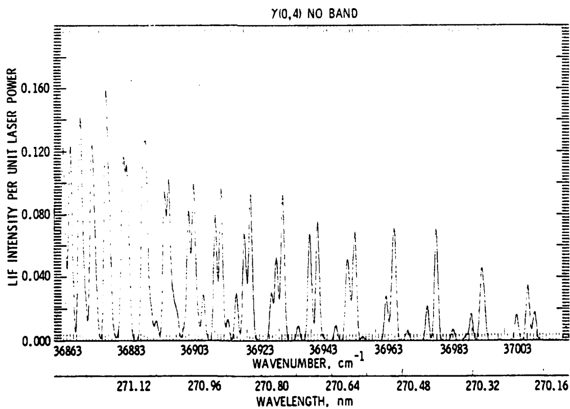
Figure 7. Calculated \gamma(0,4) Excitation Spectrum
