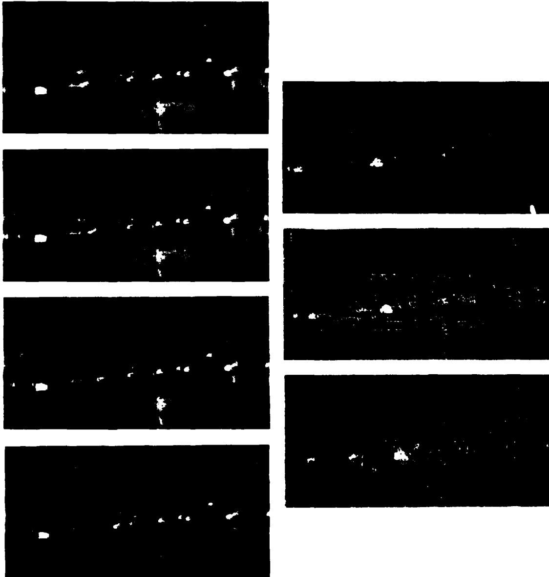
FIGURE 6 - Subtraction of FLIR imagery. The left four photographs show a series of FLIR images, and the three on the right give the differences between successive images. The uncanceled regions in the difference images correspond to moving targets and to errors present in the left part of the third FLIR image.
