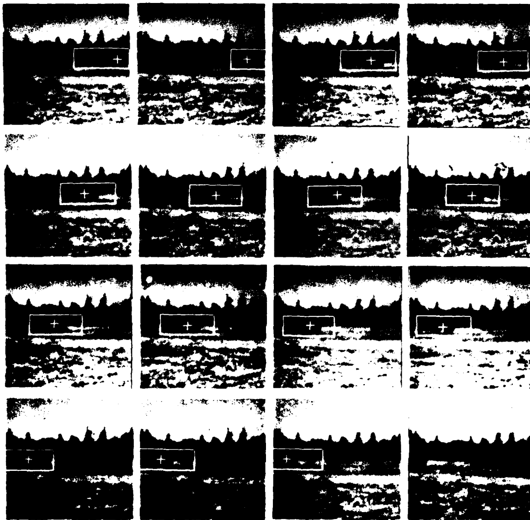
FIGURE 5 - The original cinefilm sequence with the tracking window outlined and the target positions, as determined from the difference images, designated by crosses. The target is easily tracked despite its low contrast and the high image noise level.
