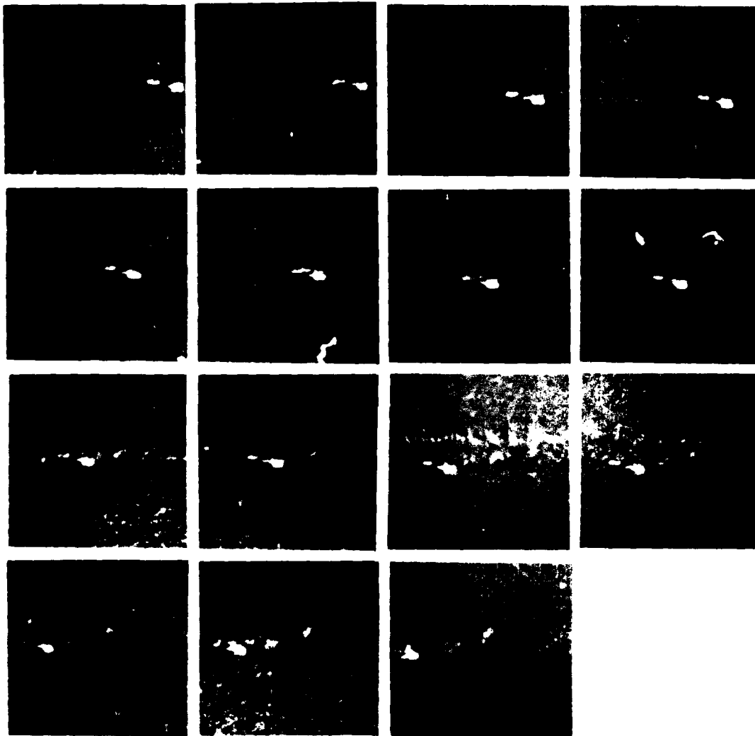
FIGURE 3 - The difference images obtained by subtracting successive images of the cinefilm sequence given in Fig. 1. The upper left photograph is Image 2 minus Image 1, the next one to the right Image 3 minus Image 2, etc. The display has been biased so that correctly cancelled regions appear gray, negative differences are dark and positive differences are light. The dark and light areas corresponding to the moving target are clearly evident.
