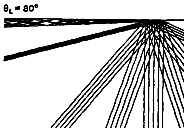
Figure 4-9. The equivalent Love ray beam in a 3^\circ updip showing leaked beams.
