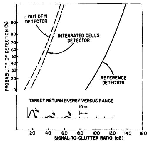
Fig. 10 - Target Model No. 8
