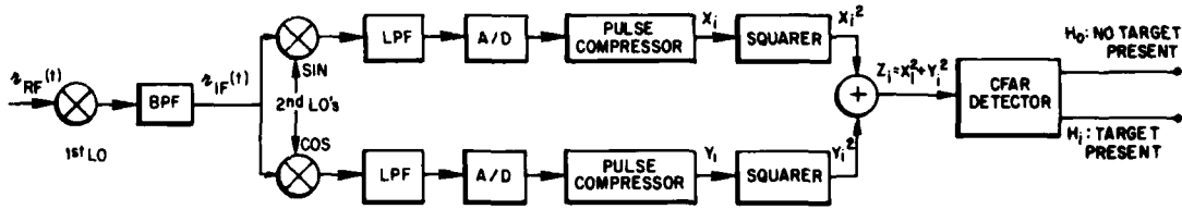
Fig. 1 — Radar receiver
