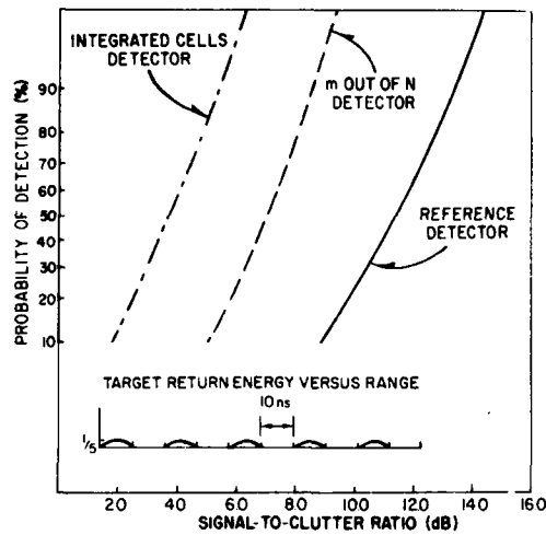
Fig. 7 - Target Model No. 5
