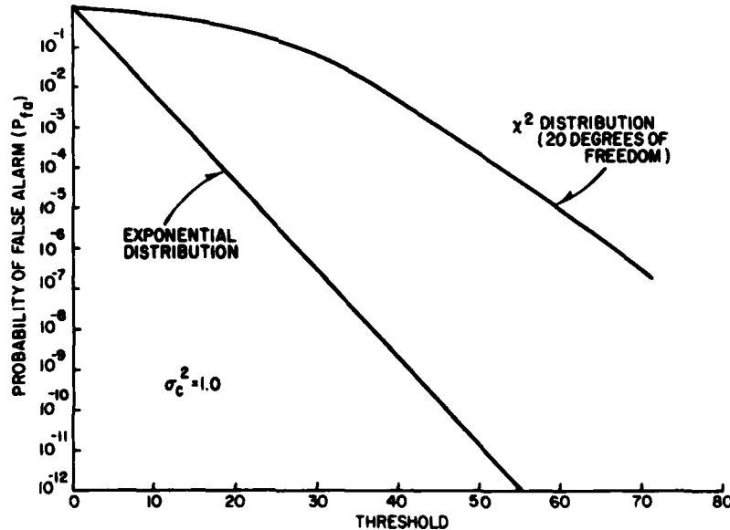
Fig. 2 — Probability of false alarm vs. threshold level
