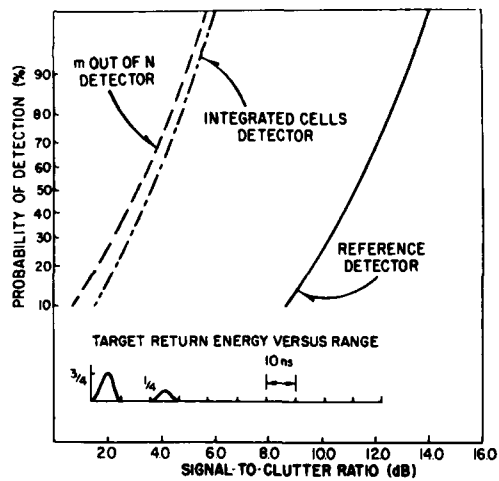
Fig. 9 - Target Model No. 7
