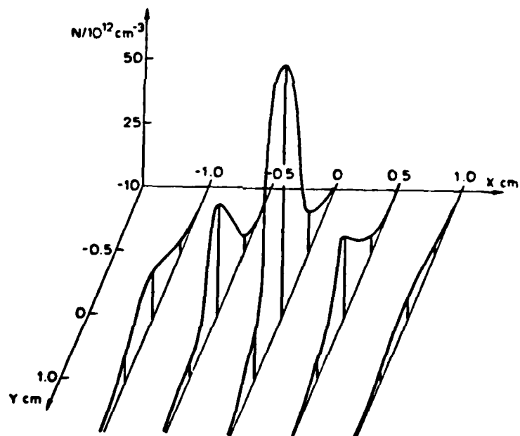
Figure 13. Sodium concentration above salt grain in z = 0.5 cm plane.
