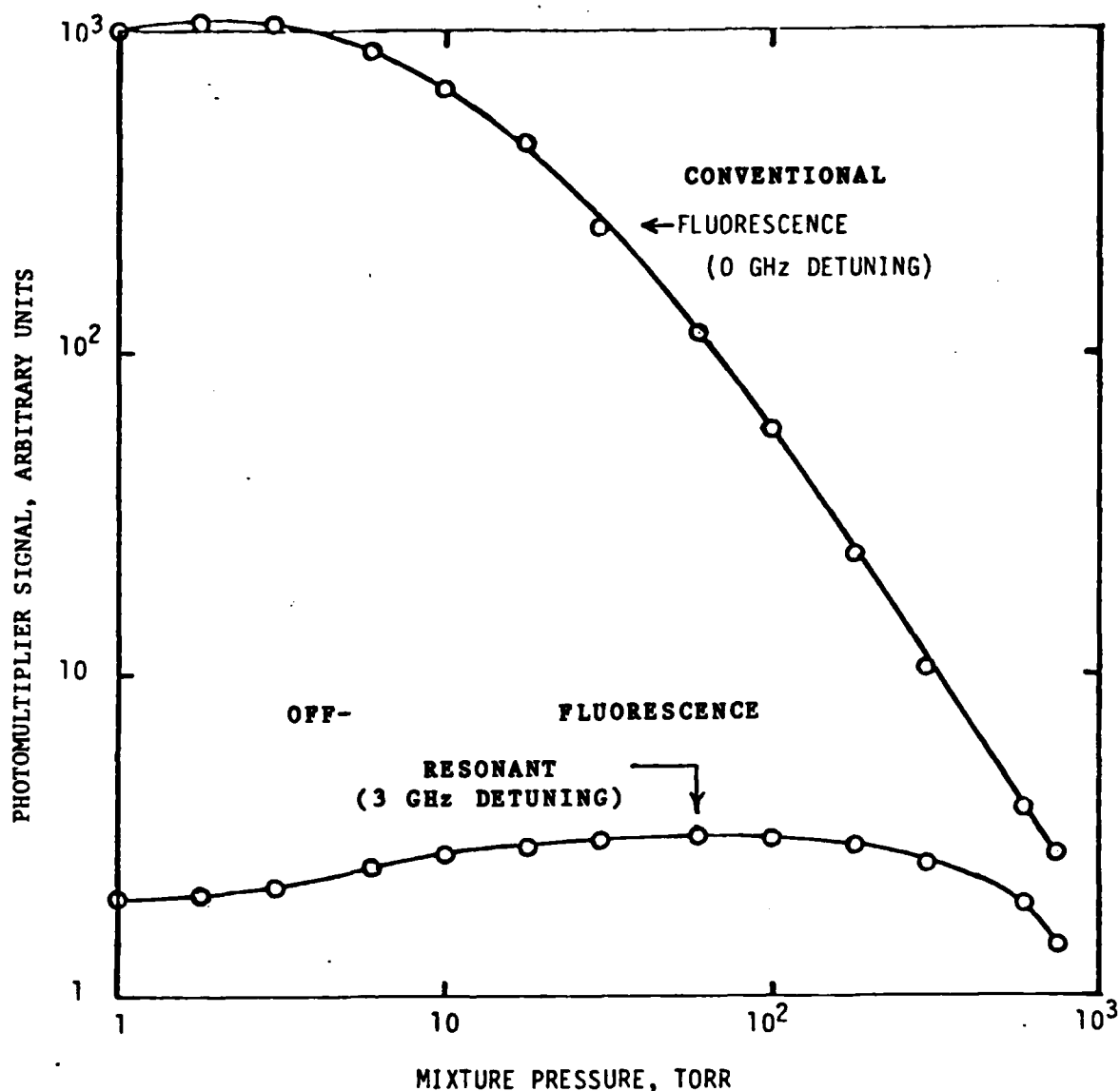
Figure 23. Reduced effects of quenching with increasing detuning between the frequency of the laser excitation and an absorption line in iodine; partial pressure of iodine = 0.3 torr; 514.5 nm argon-ion wavelength.
