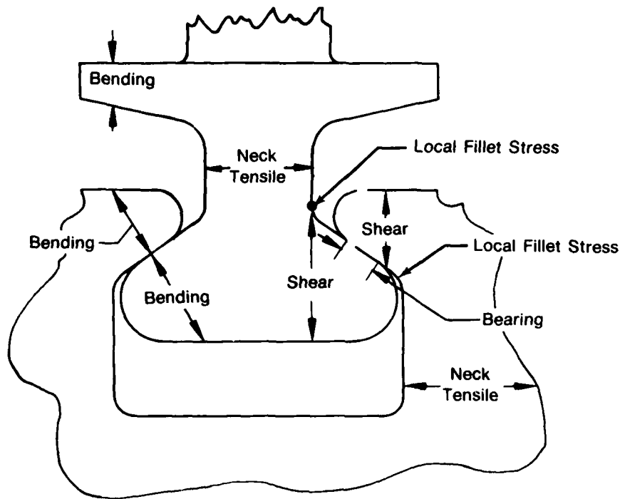
Figure 2-4. Blade/Disk Attachment Design Criteria Summary.
