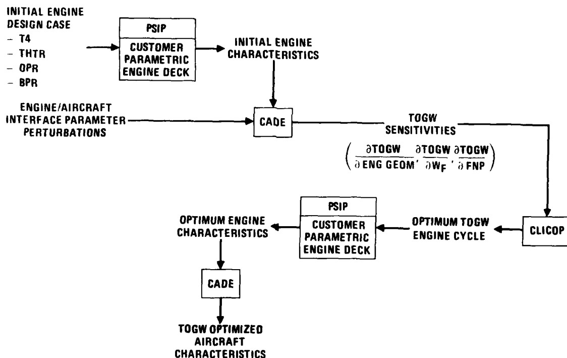
FIGURE 31 ENGINE CYCLE OPTIMIZATION PROCEDURE
