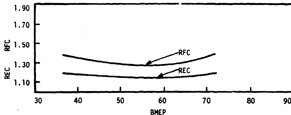
FIGURE 9f. RFC AND REC VERSUS BMEP FOR DF-2 EMULSION WITH 10% CARBON AT 2000 RPM
