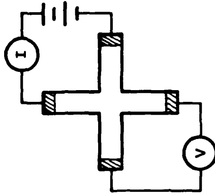
4-POINT MEASUREMENT
