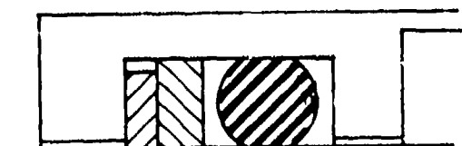
Figure 14. Backup Candidate B19; TF830-214-1 and TF830-214-2 Two Stage Backup
