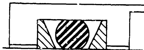
Figure 18. Backup Candidate B23; S32975-214-20
