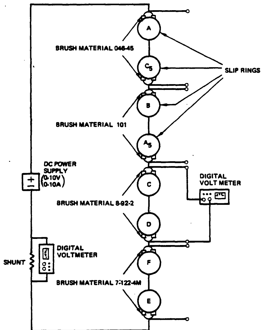
Figure 2. Test Circuit Schematic
