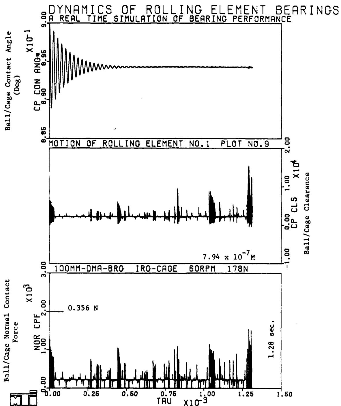
Fig. 4-5 Ball Cage Interaction for the 100 mm DMA Ball Bearing
