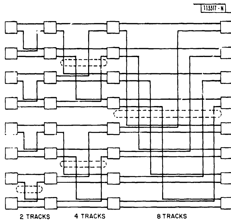
Fig. 5. FFT network.
