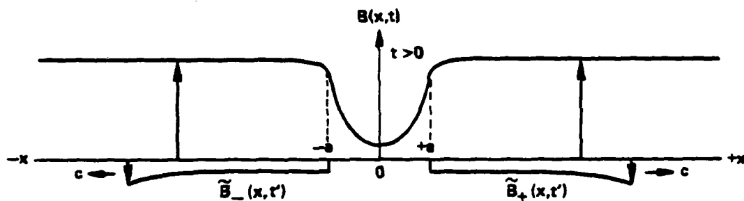
FIG. 2: Diffusion Field B(x,t) and Transients \tilde{B}_\pm(x,t) for t > 0 and t' > 0 (qualitative).
