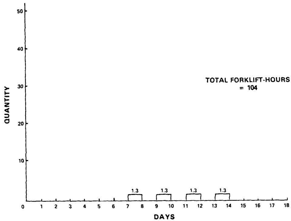
Figure 8-12. Forklift Utilization
