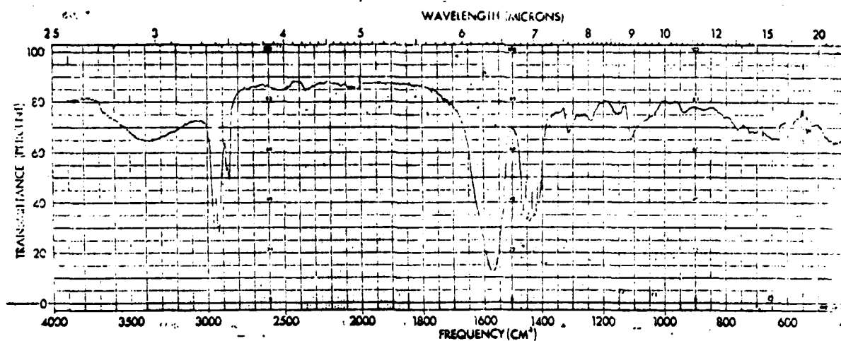
Figure 25. Infrared Spectrum of (\text{Mg C}_{10} \text{H}_{20} \text{O}_4)_x .
