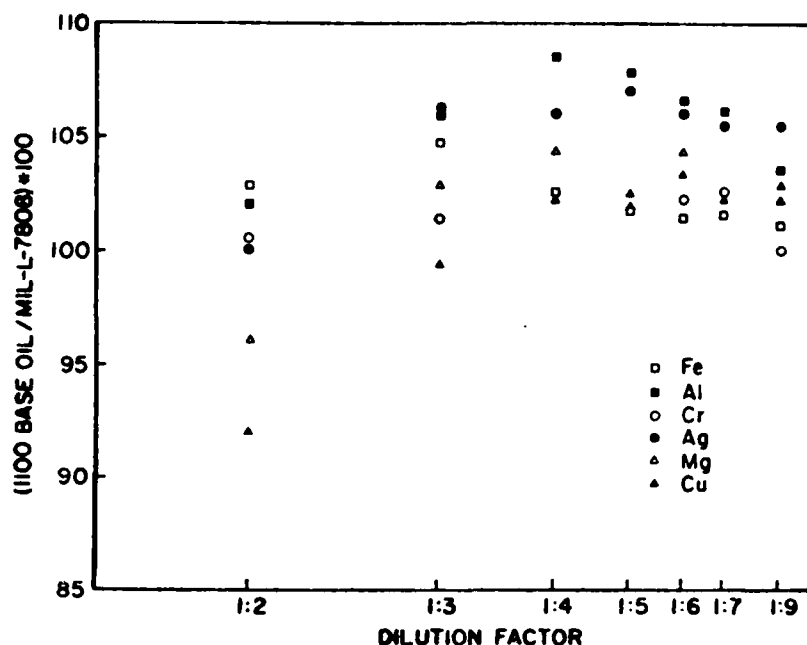
Figure 30. Effect of Dilution on the Absorbances for D20 Conostan Standards in 1100 Base Oil and MIL-L-7808 Ester Oil
