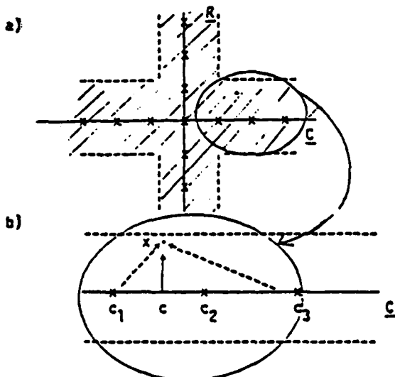
Figure 2: a) Solution space under a single failure assumption. b) Illustration of the differential-interpolative diagnosis algorithm.
