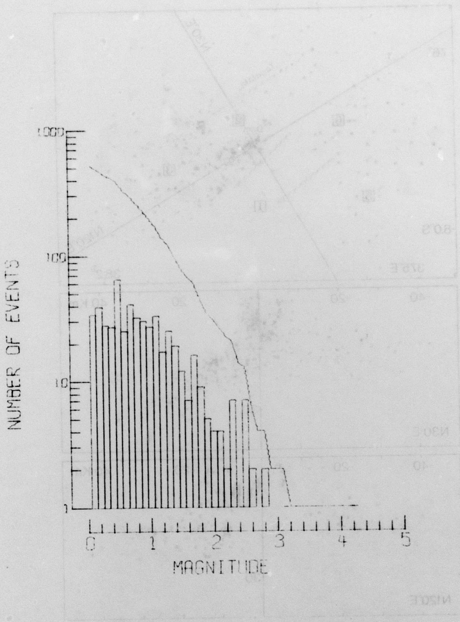
Fig. VI.7.3 Frequency-magnitude distribution for local earthquakes recorded by SGSN. Corresponding epicenter locations are given in Fig. VI.7.1.
