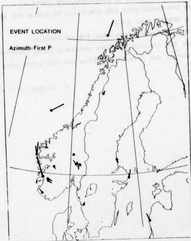
Fig. VI.2.1 'Location errors' using NORESS (with azimuths determined from the first P phase) for regional event location. Dots indicate epicenters determined by the Fennoscandia station network, while the end of the arrows indicate locations from NORESS processing.
