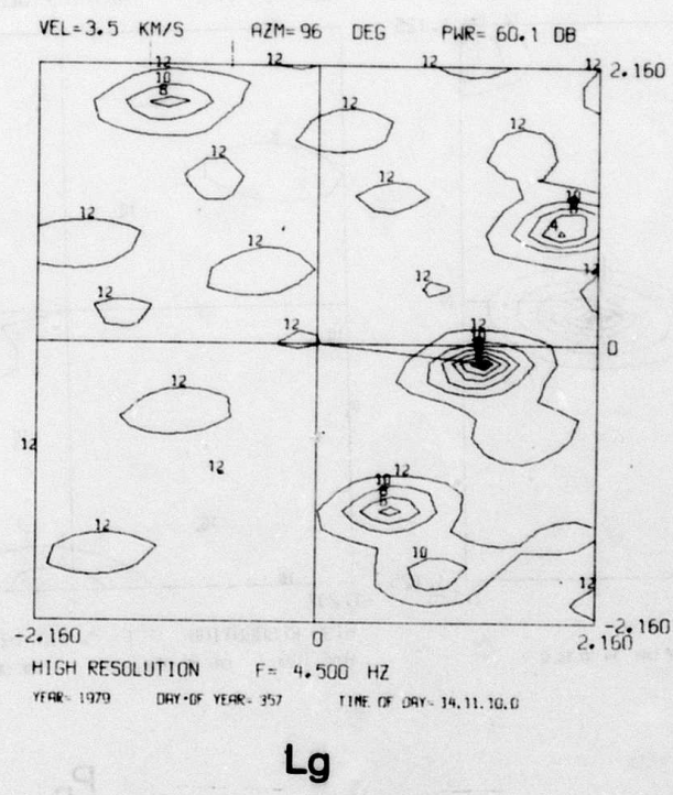
Fig. VI.1.9 Same as Fig. VI.1.8 for two frequencies for the Lg phase.
