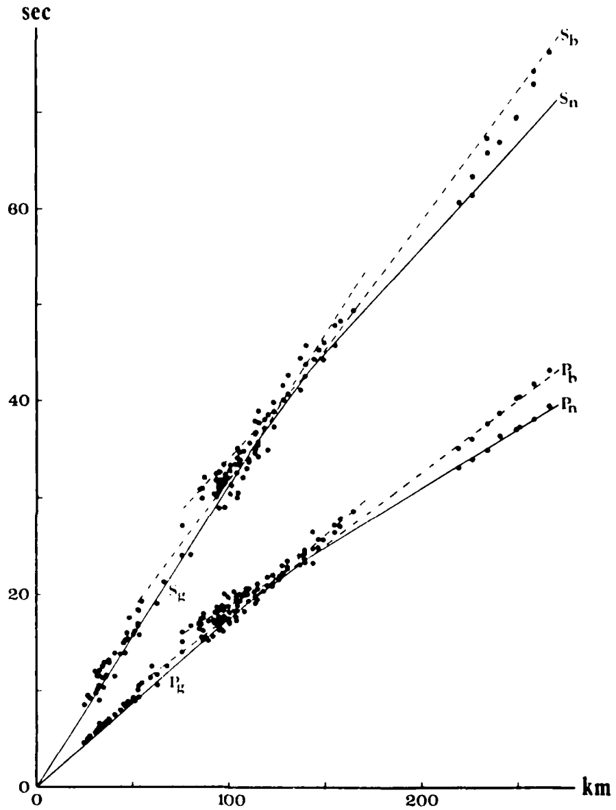
Fig. v1.6.1 Continental travel times for Svalbard, with dots giving travel times (vs distance) for explosions, and straight lines travel times computed from the derived model. Most of the readings are from PRD, some from KBS and a few from SWE.
