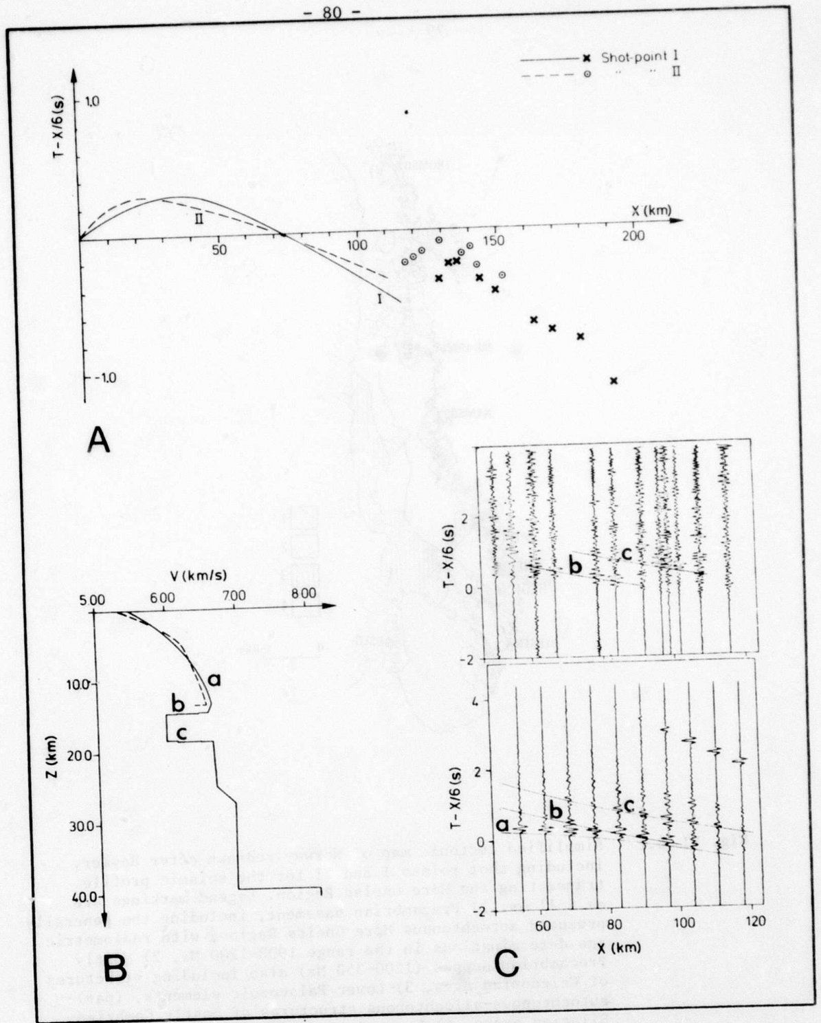
Fig. VI. 5.2 A) First arrival travel times for both shot points. The continuous curves represent a slight smoothing of travel time observations. B) Velocity-depth distribution derived from shot point I data. The dashed curve corresponds to shot point II data. C) Detail of record section (top) for shot point I and corresponding synthetic section (bottom). Selected segments of the travel time curves as computed from Fig. VI.xx.2b are inserted.
