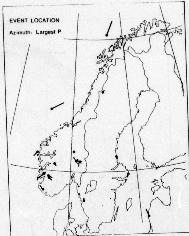
Fig. VI.2.2 Same as Fig. VI.2.1, but with NORESS azimuths determined from the largest P phase.
