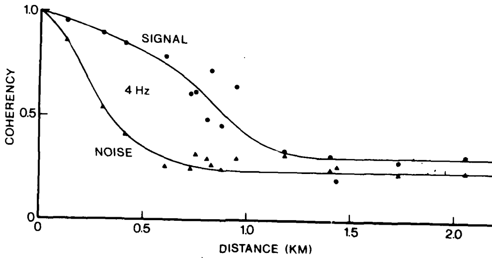
Fig. VI.1.5 Same as Fig. VI.1.4, for 4 Hz.
