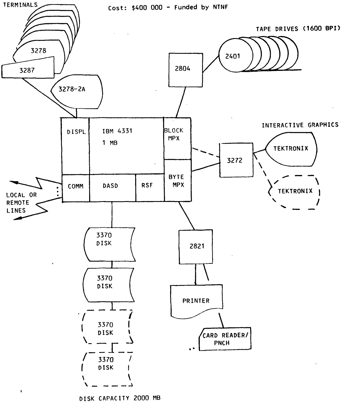
Fig. III.2.1 The IBM 4331 research computer system at NORSAR.
