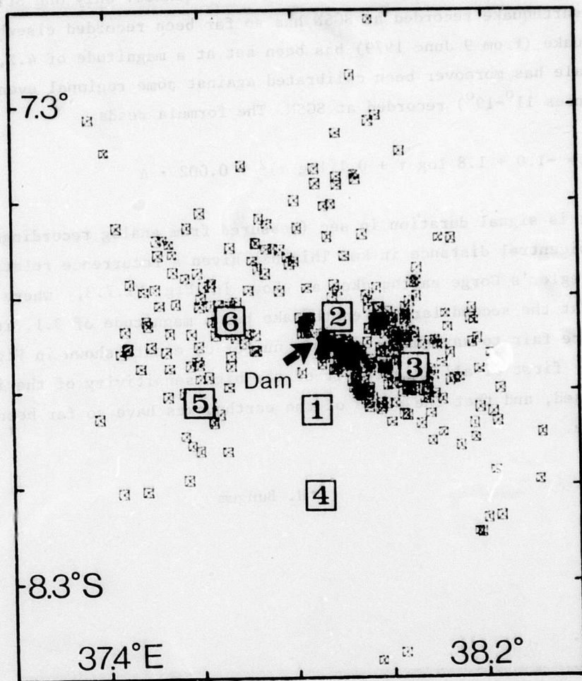
Fig. VI.7.1 Precisely located earthquakes in the Stiegler's Gorge area between 14 Sep 1978 and 16 Jan 1980. The locations of the seismic stations (SGSN) are given as boxed numbers.
