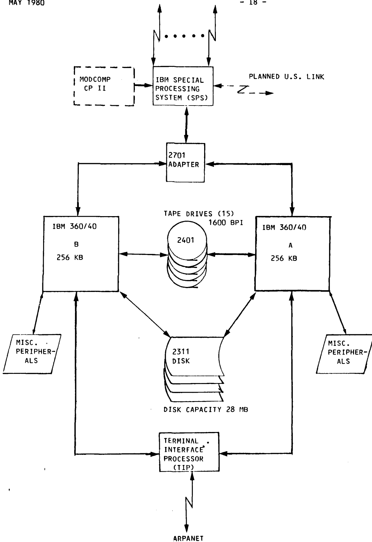
Fig. III.1.1 Current NORSAR on-line computer configuration.
