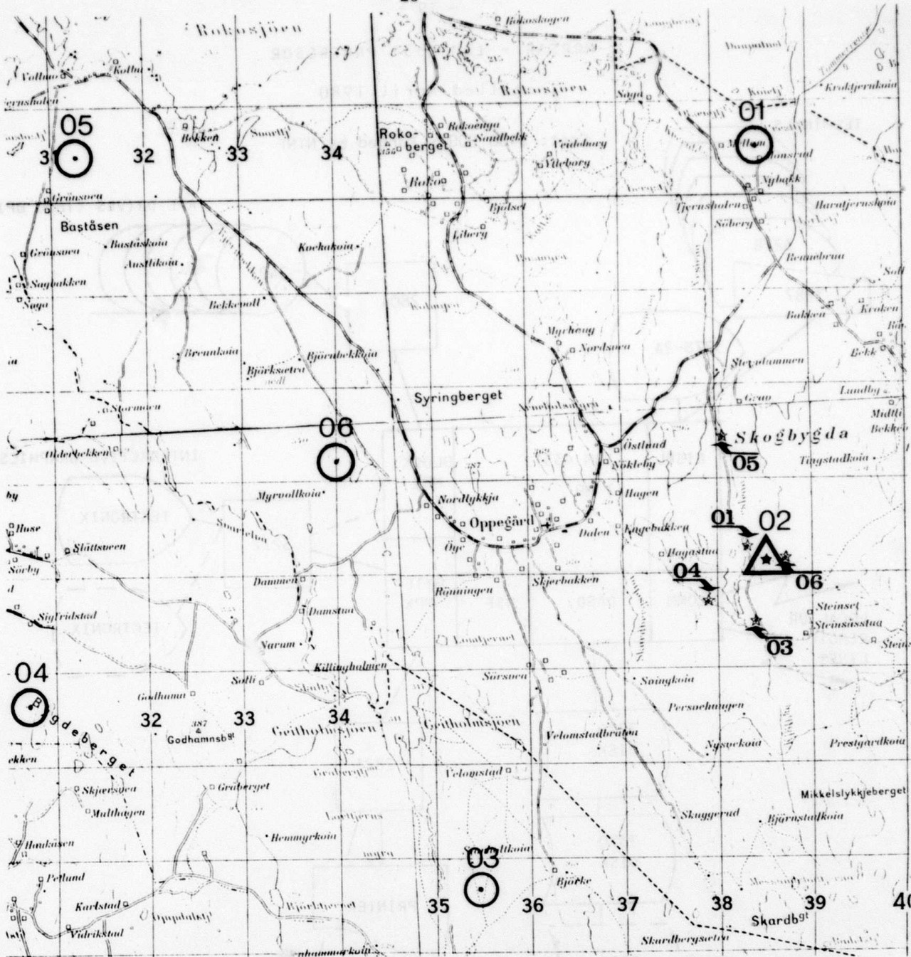
Fig. III.3.1 Configuration of subarray 06C including the experimental small subarray (NORESS - NORSAR Experimental Small-Aperture Subarray) marked with arrows. 06C02 (LPV) and NORESS 02 are common. In operation from 16 October 1979, substituting subarray 06C. From 27 March 1980 both subarrays are in operation, NORESS substituting 01B data.
