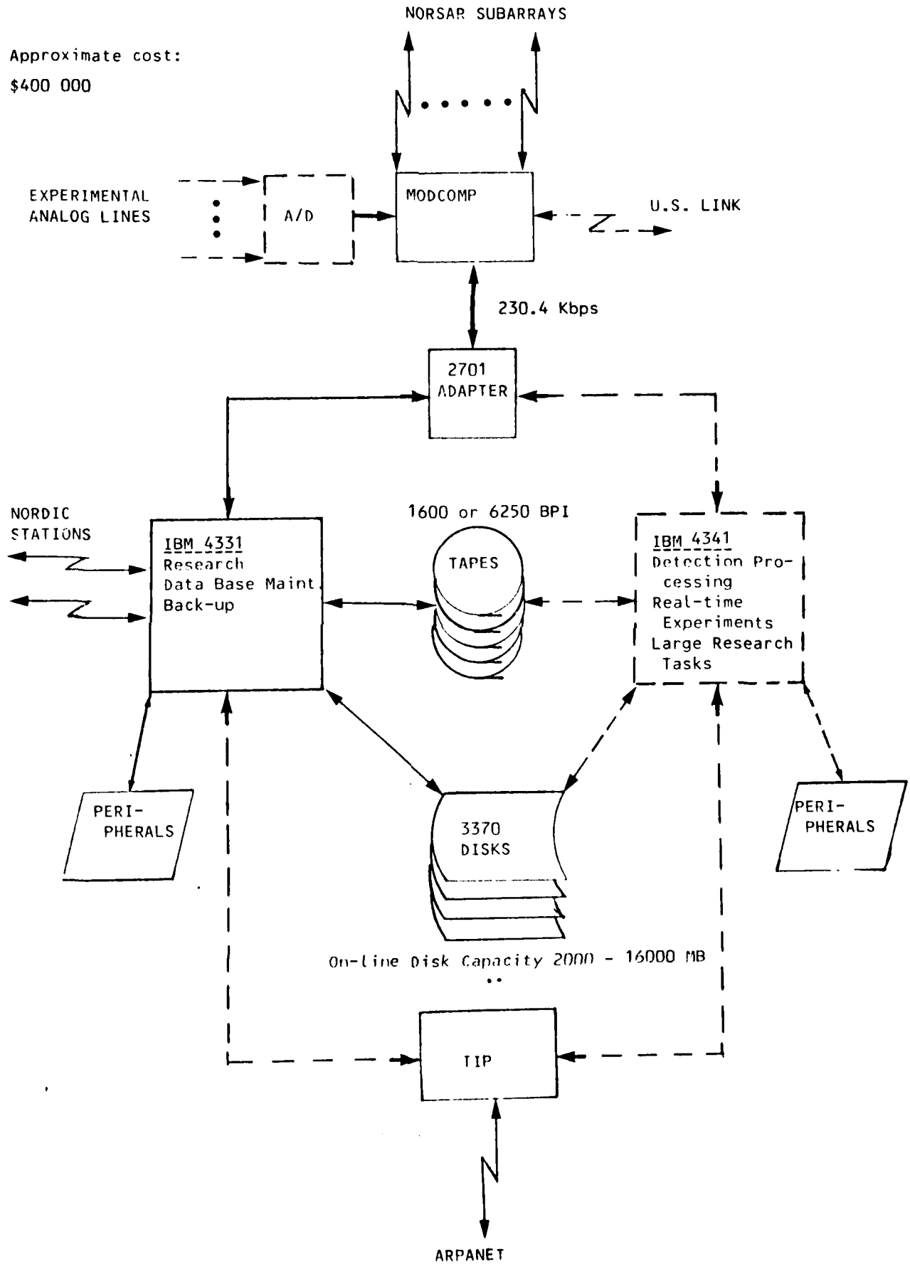
Fig. III.5.1 Suggested future NORSAR computer configuration.
