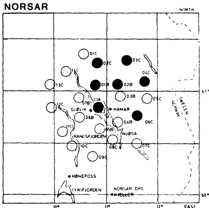
Fig. VI.6.1 Deployment of the original 22 NORSTAR subarrays (from 1971 to October 1, 1976). The subset of 7 subarrays in operation since October 1, 1976, are marked as filled circles.
