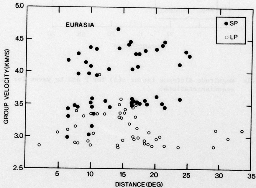
Fig. VI.7.2b Same as Fig. VI.7.2a for stations in Central Asia.
