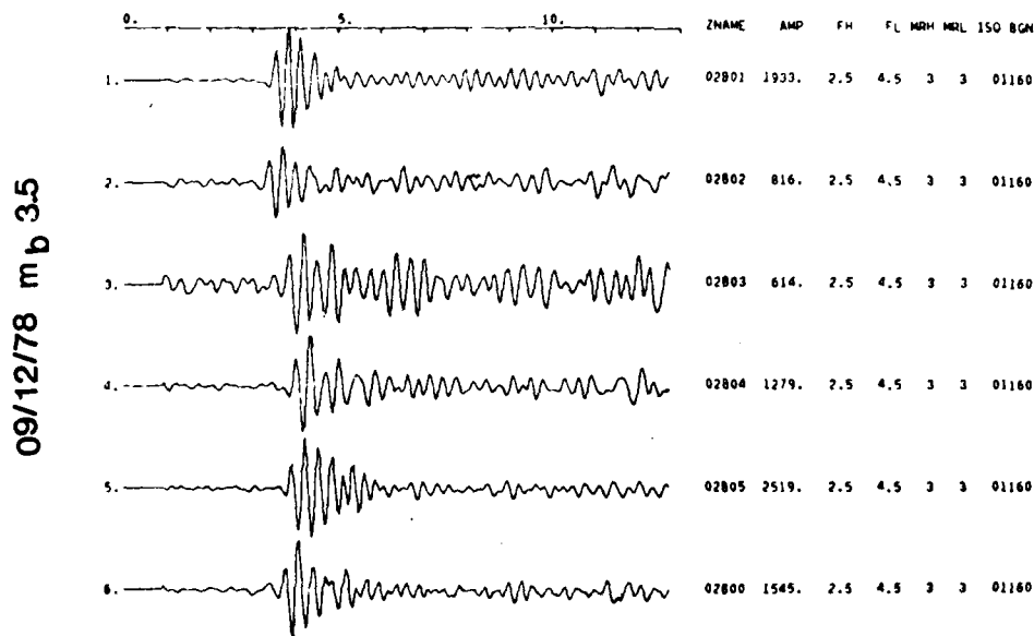
Fig. VI.6.2 NORSTAR-recorded signals (at subarray 02B) for Event 9 in Table VI.6.1. The signals have been bandpass filtered (2.5-4.5 Hz) and are scaled to max. amplitude for each of the six sensors. Note the significant variation in amplitude (a factor of 4) across the subarray, from 614 q.u. at 02B03 to 2519 q.u. at 02B05.
