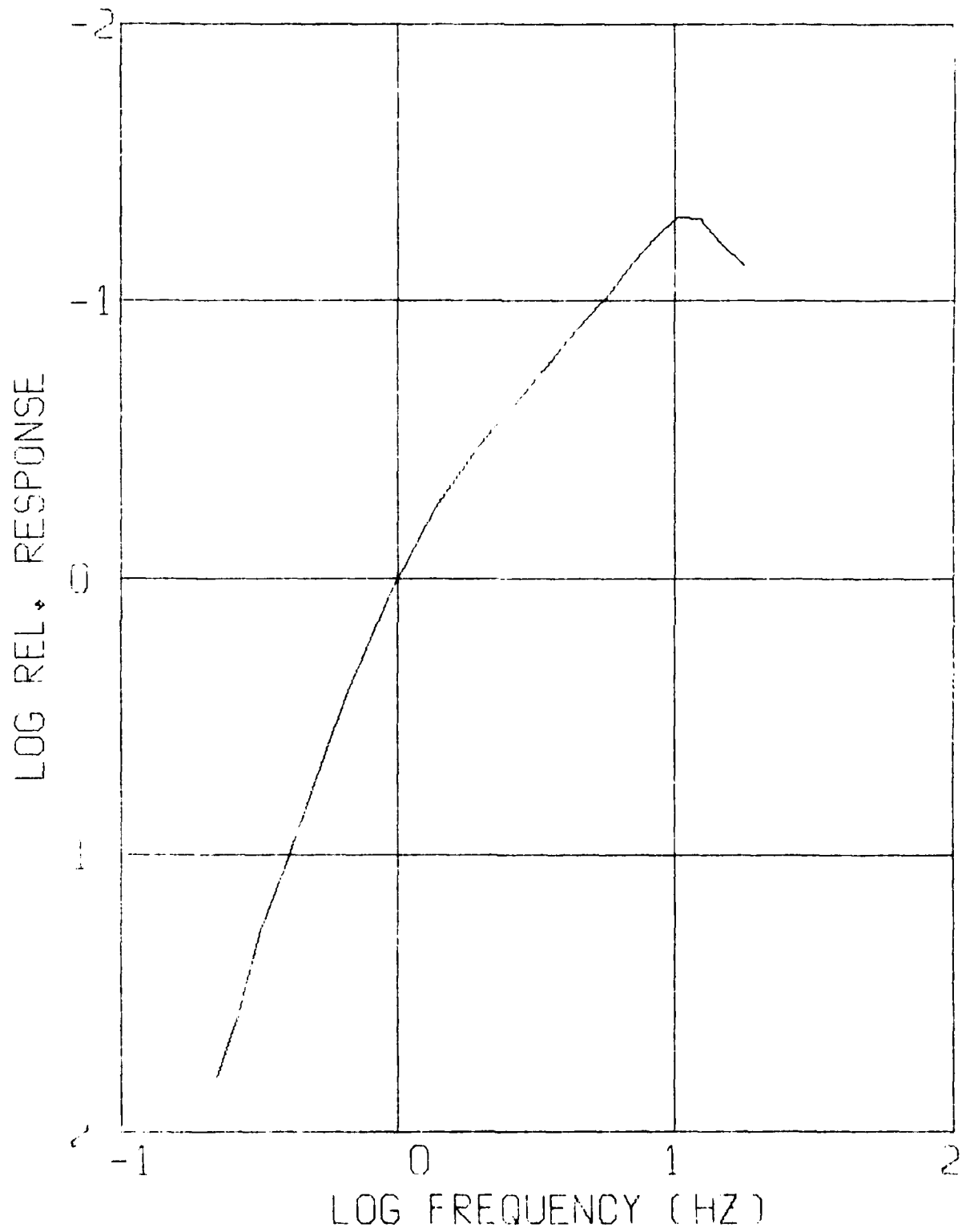
Fig. III.4.2 Southern Norway Seismic Network relative response.
