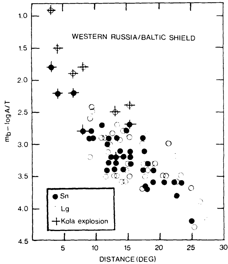
Fig. VI.7.3b Same as Fig. VI.7.3a for Lg and Sn waves.
