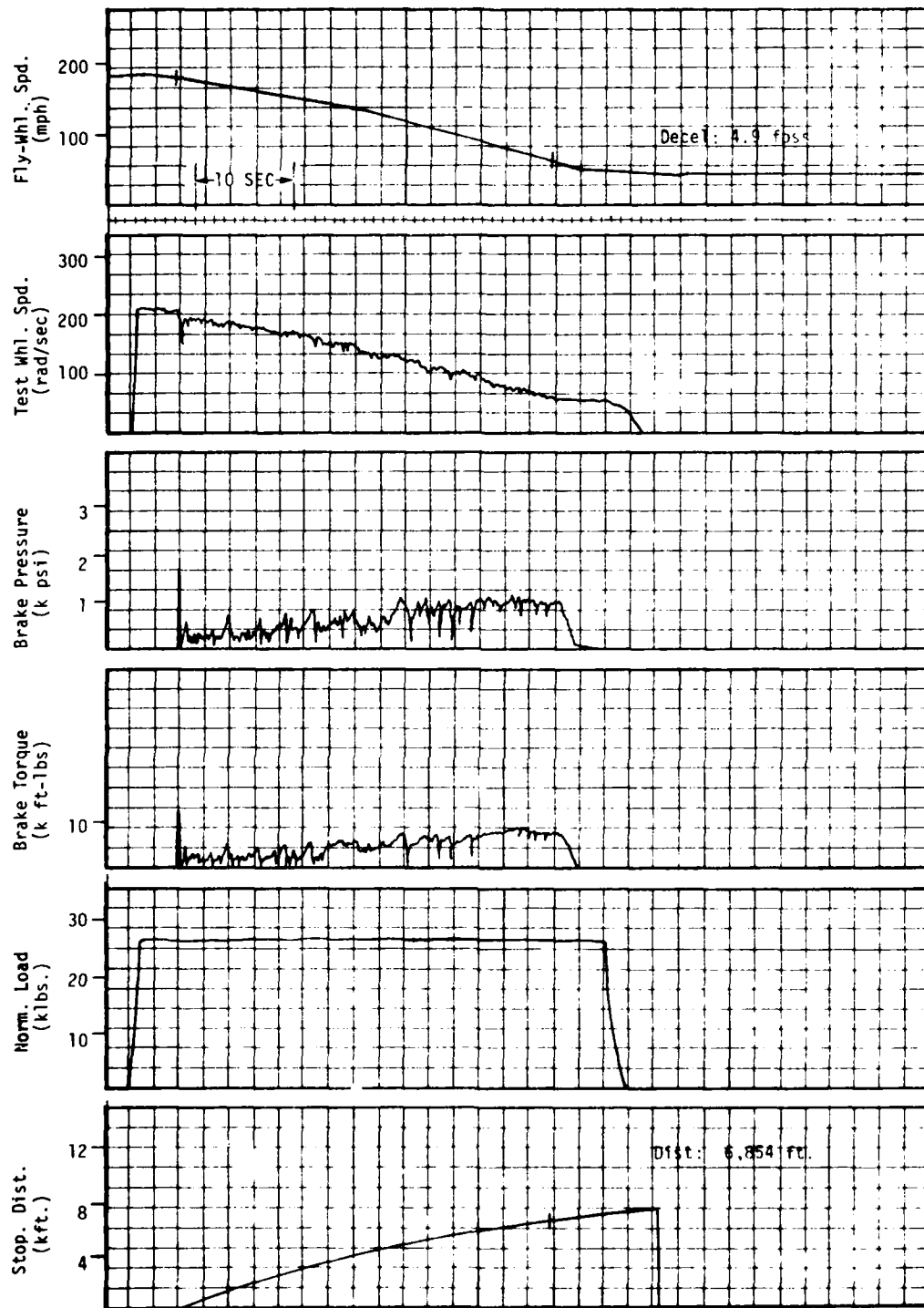
Figure C-29. S/N1293(22-N), Siped 3/16" X 8/32", Cyl. 77, 1.0 gpm
