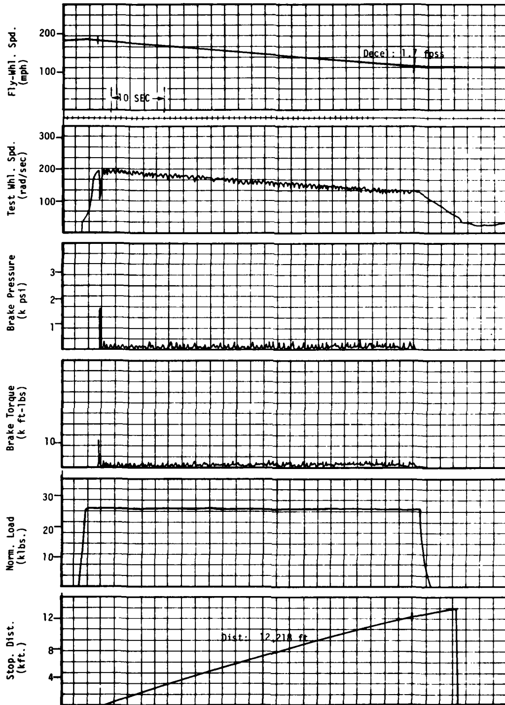
Figure C-15. S/N1174(20-N), Siped N/A, Cyc. 63, 2.0 gpm
