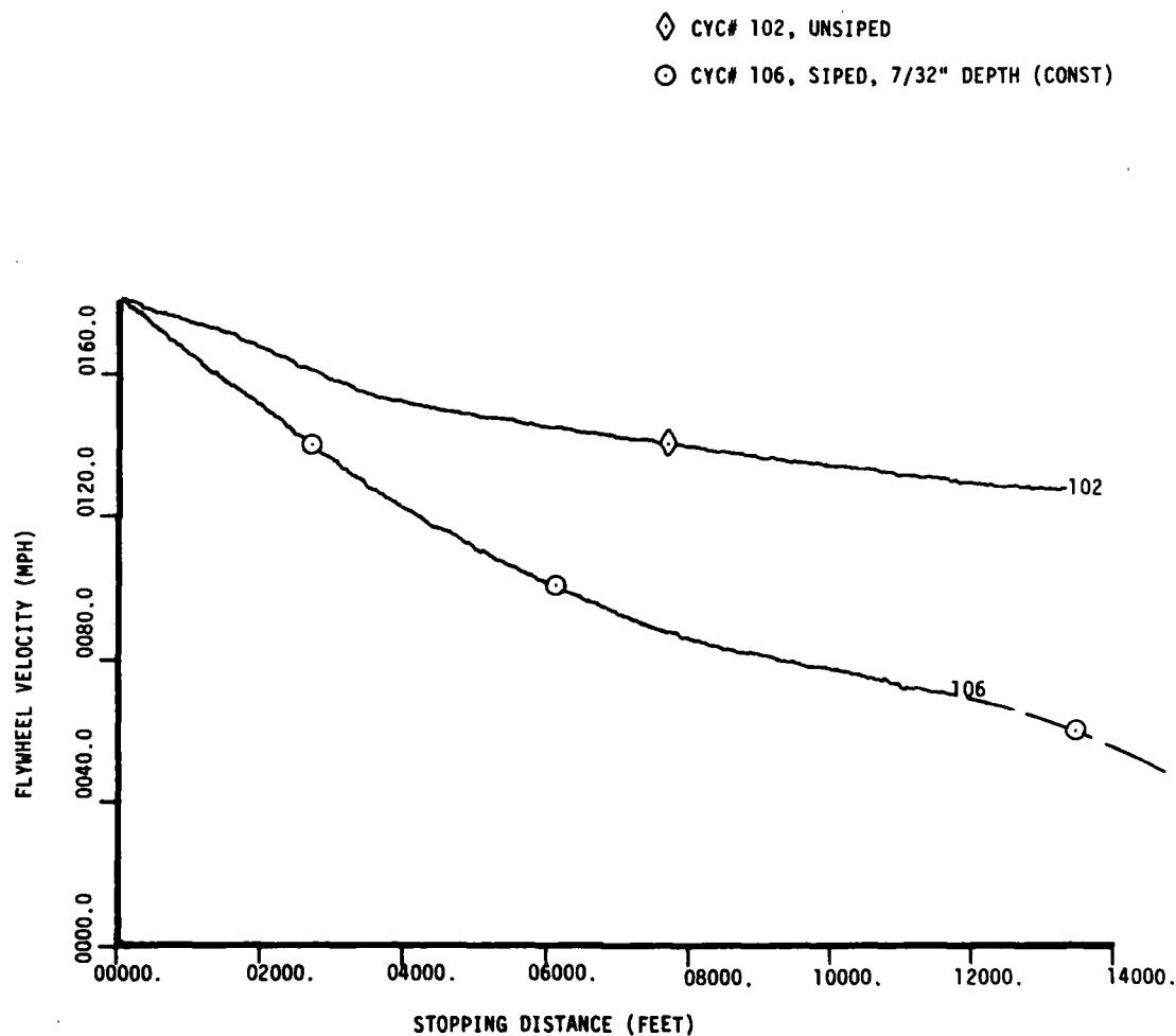
Figure D22. Velocity vs. Brake Distance F-4 MLG, Siped Tire Evaluation 16,000 (LBS) Tire Load, 1.0 (GPM) Flow Rate Code Number 1-R-2 Water On After Landing
