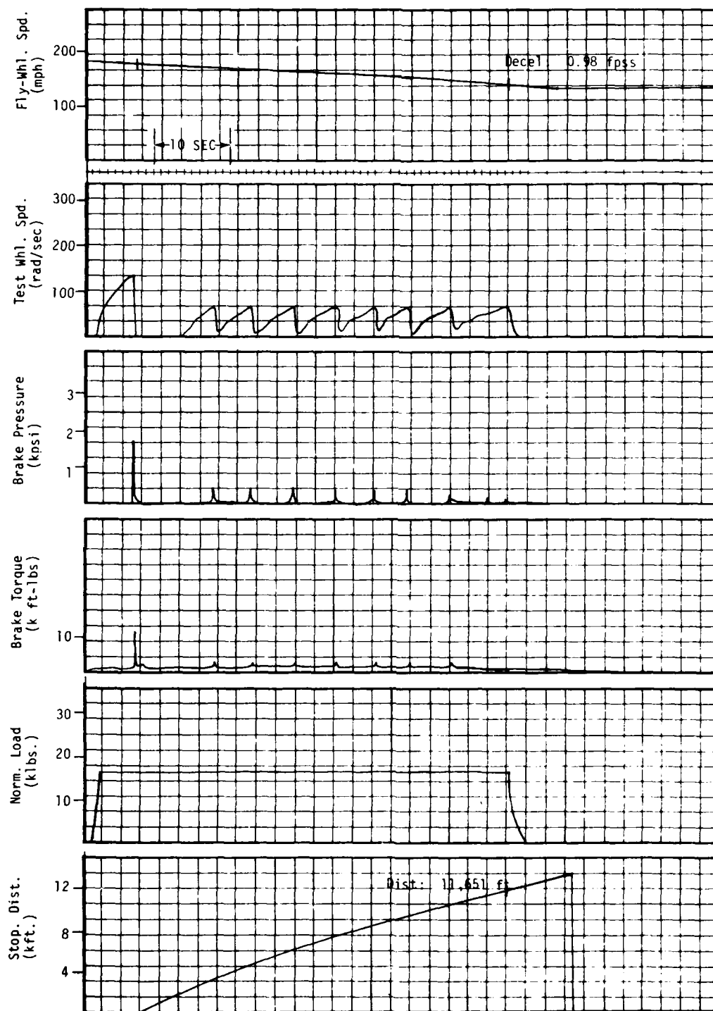
Figure C-34. S/N6A0013(#1-R-2), Siped N/A, Cyc. 98, 2.0 gpm
