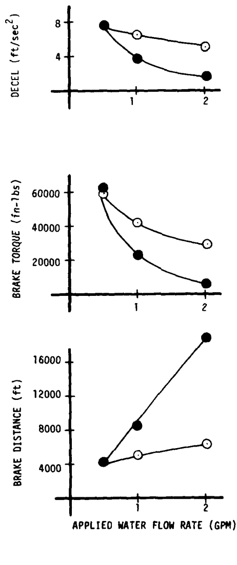
Figure 36. Brake Stop Data vs Water Flow Rate, Tire Code Number 20-N
