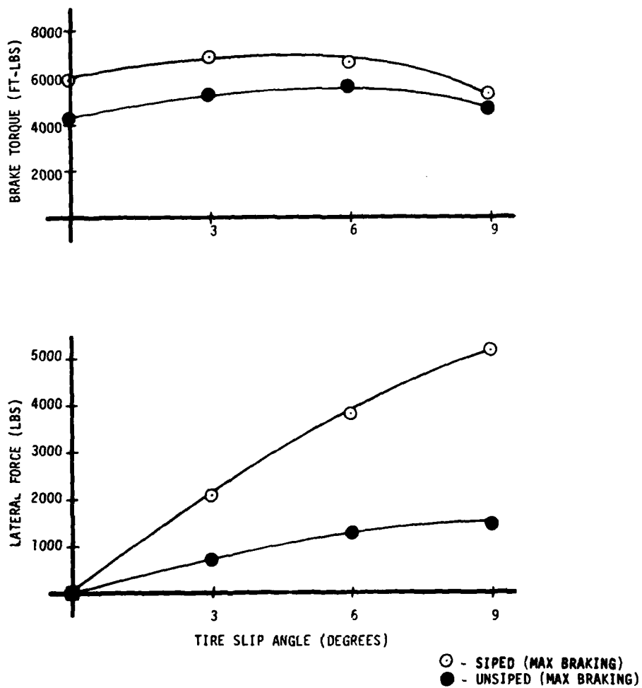
Figure 21. Brake Torque and Lateral Force vs Slip Angle, Flooded Surface, Tire Code Number 3-N (Siped 8/32" Deep X 3/16" Spacing)
