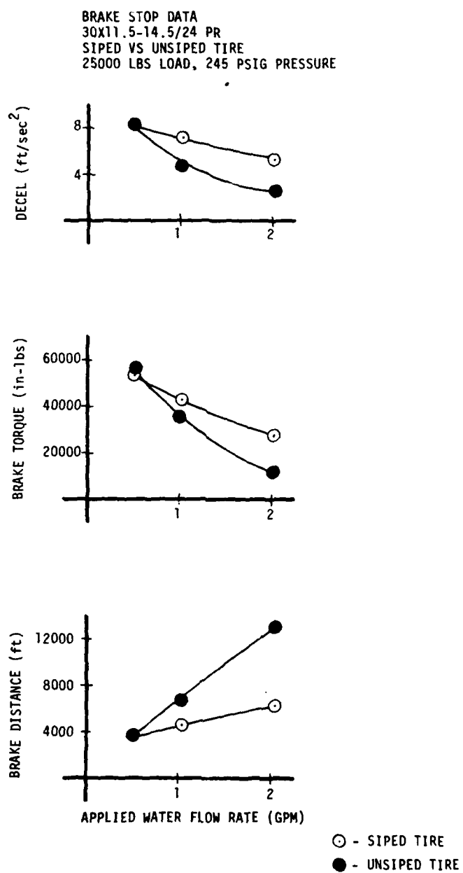
Figure 38. Brake Stop Data vs Water Flow Rate, Tire Code Number 21-N
