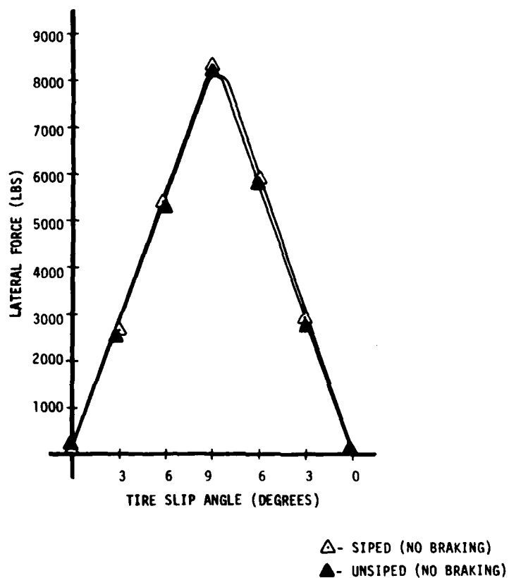
Figure 33. Lateral Force vs Slip Angle, Dry Test Surface, 30 MPH, Tire Code Number 24-N (Siped 8/32" Deep X 3/16" Spacing)
