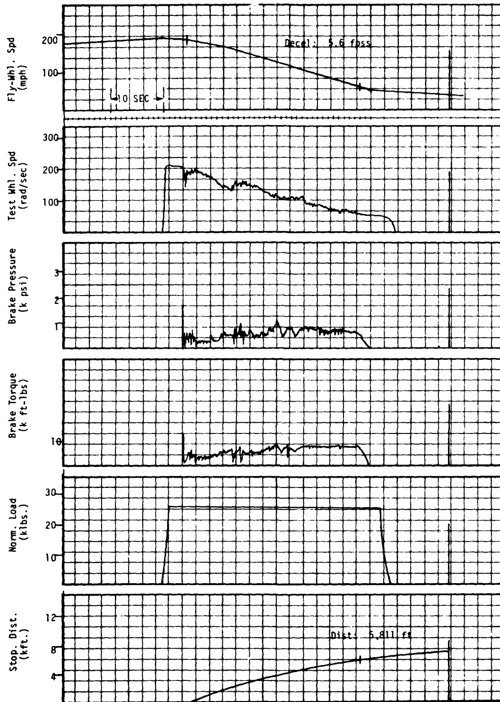
Figure C8. S/N0870(18-N), Siped 3/16" X 8/32", Cyc. 56, 1.0 gpm
