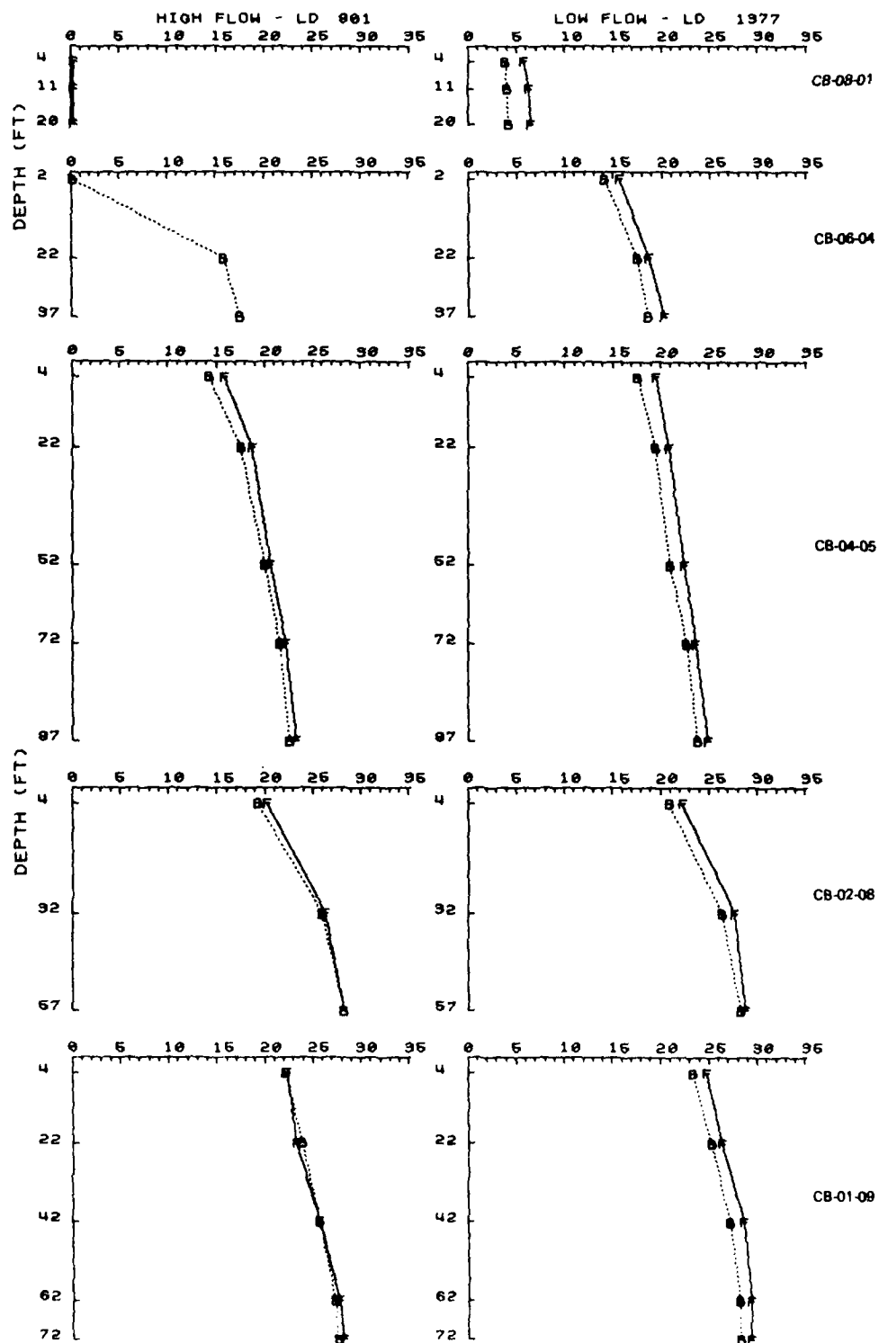
Plate 101. Salinity profiles, sta CB-08-01, CB-06-04, CB-04-05, CB-02-08, and CB-01-09, lunar days 901 and 1977
