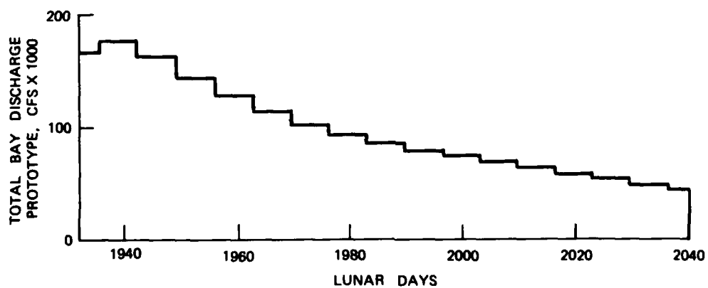
Figure 14. Lunar days 1932-2040 at sta CB-01-09 showing salinity changes with tide amplitude
