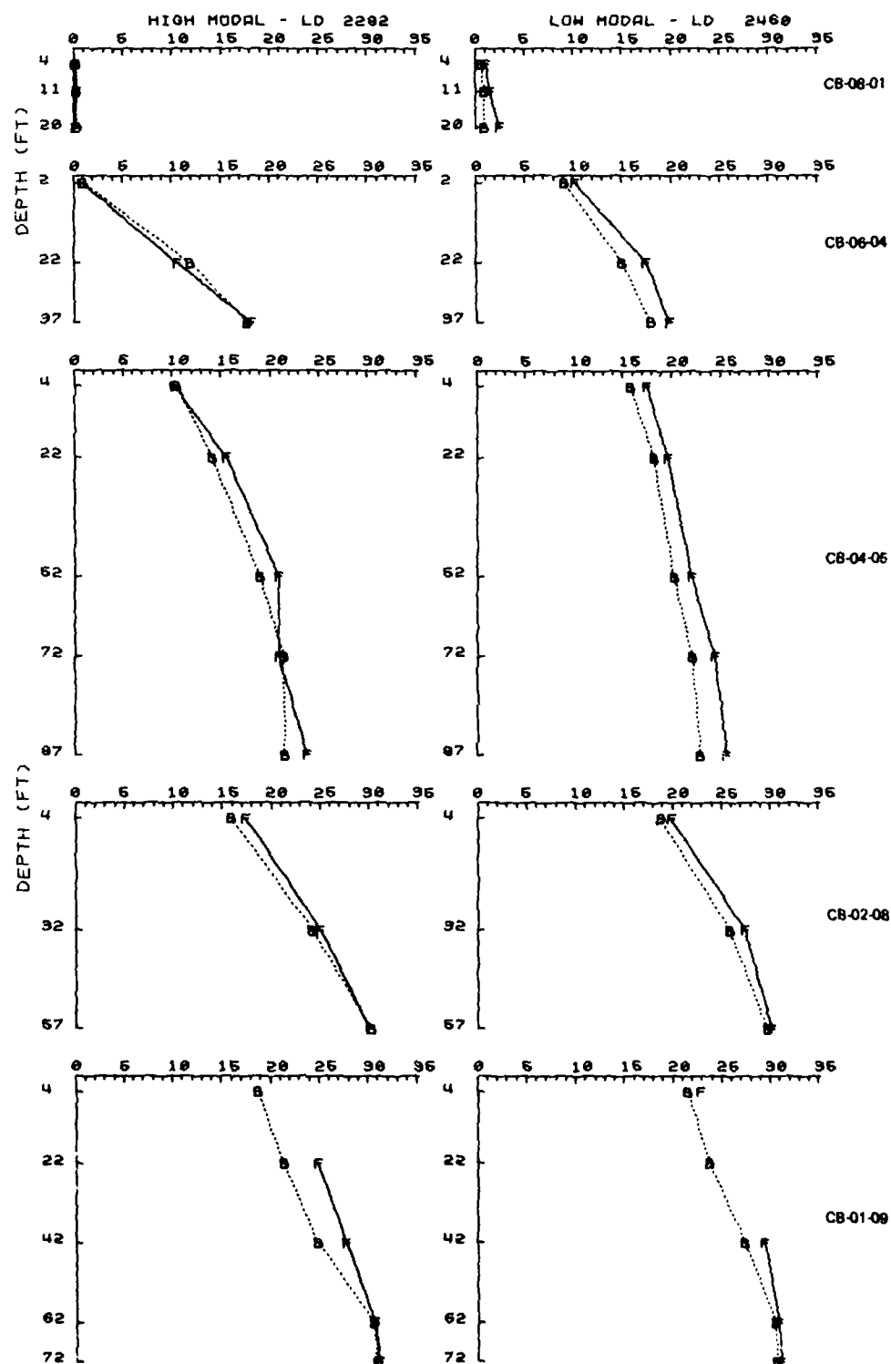
Plate 107. Salinity profiles, sta CB-08-01, CB-06-04, CB-04-05, CB-02-08, and CB-01-09, lunar days 2292 and 2460
