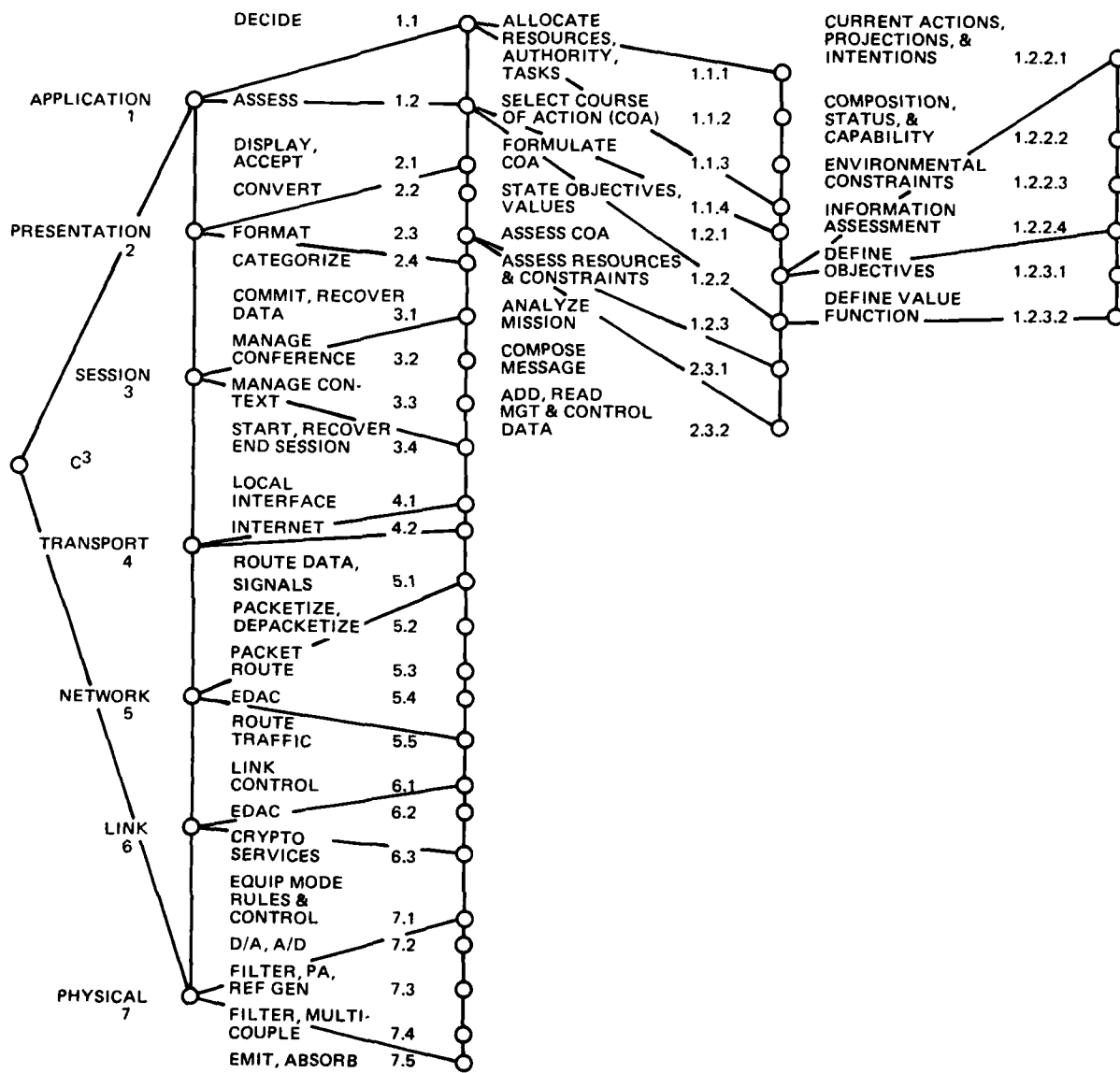
Figure 3-1. C³ system layered breakdown structure.
