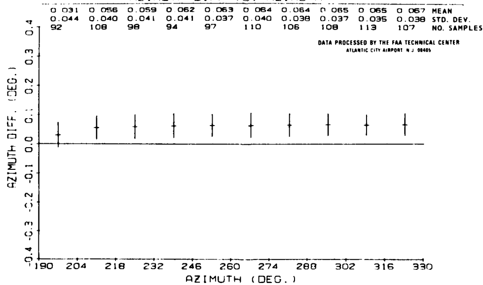
FIGURE 8. AZIMUTH RESIDUAL VERSUS ELEVATION AND AZIMUTH PLOTS FOR TECHNICAL CENTER ORBITAL FLIGHTS OF JULY 22, 1980 (SHEET 2 OF 2)
