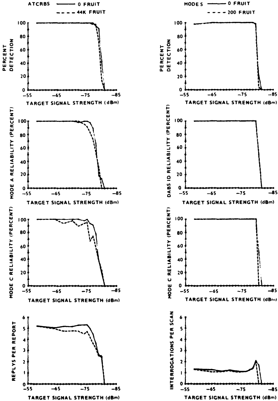
FIGURE 9. ATRCBS/MODE S PERFORMANCE AS A FUNCTION OF SIGNAL STRENGTH
