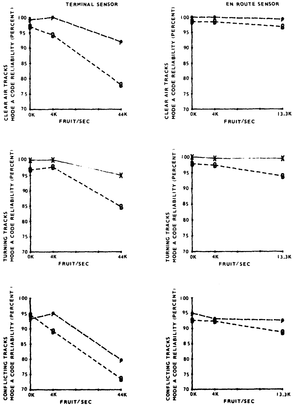
FIGURE 19. MODE 3/A CODE RELIABILITY (ATCRBS) TERMINAL VERSUS EN ROUTE SENSOR, EFFECTIVE BEAM WIDTH 3.4°
