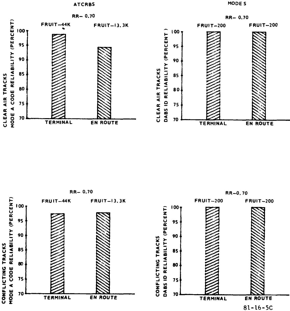
FIGURE 5. ATCRBS MODE 3/A MODE S ID RELIABILITY — TERMINAL VERSUS EN ROUTE SENSOR, EFFECTIVE RECEIVE BEAM WIDTH 2.4° (Sheet 3 of 3)
