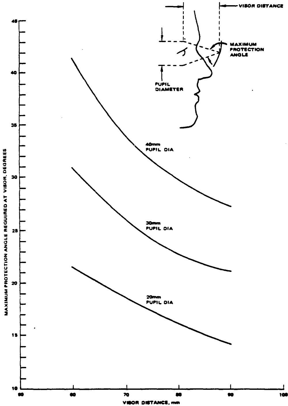
Figure 7. The angular range over which the designated wavelength must be adequately shielded is large when the shielding surface is close to the eye.
