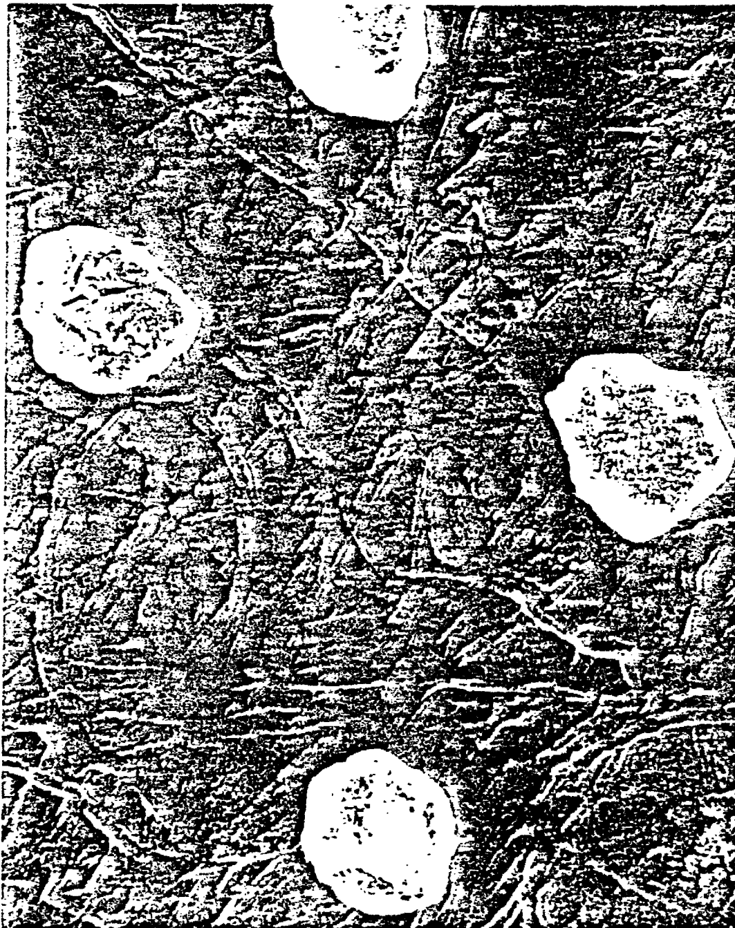
Figure 42. SEM photograph of four particles collected from the p = 1.0 , T_f = 1683 K, d_{po} = 52.6 \mu\text{m} test condition at a distance of 1.3 mm from the injector.
